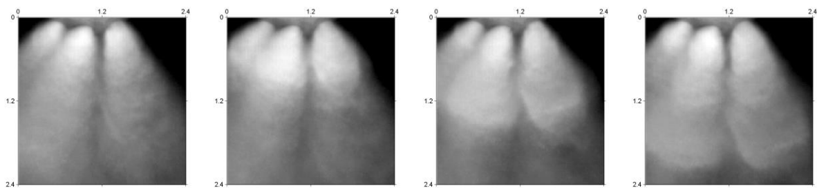
Figure 4.a-d. A rare spray flapping event across all visible nozzles of injector 2 at its lowest likely working pressure of 40 bar, shown in time steps of 10 \mu s.
