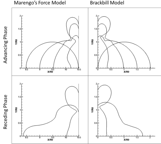
Figure 7. Temporal evolution of the impingement process for Case 3 of Table1. Results of the isoline of VOF = 0.5 are depicted for t=0, 0.9, 1.9, 3.9\text{ms} (advancing phase), and t=4.7, 8.4\text{ms} (receding phase).
