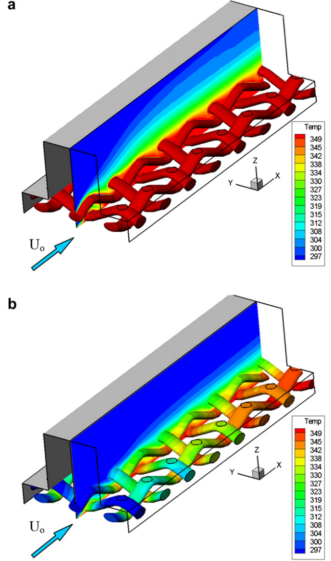
Fig. 9. Contours of constant temperature on the fibres and an XZ plane at Y/Y_{\text{tot}} = 0.25 for U_0 = 8.4 ms ^{-1} . a) Constant temperature imposed at fibres' surface, b) Conjugate temperature solution through the solid fibres with the properties of carbon cloth (ELAT). (Domain has been mirrored across XZ plane and the bipolar plate walls removed, for clarity).
