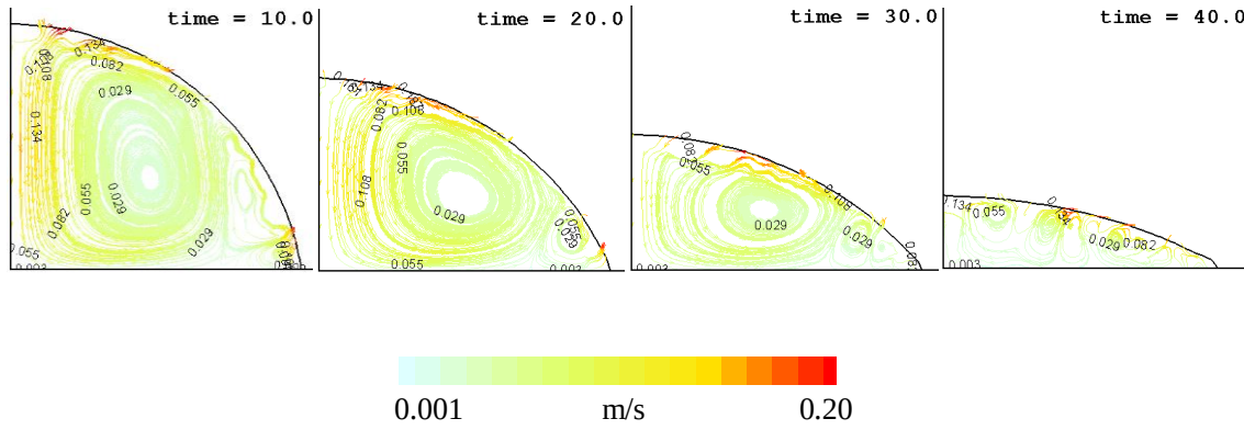
Figure 9: Predicted streamlines within the liquid during the vaporisation process using the full solution. [Initial surface temperature 80^{\circ}\text{C} , initial contact angle 90 degrees]
