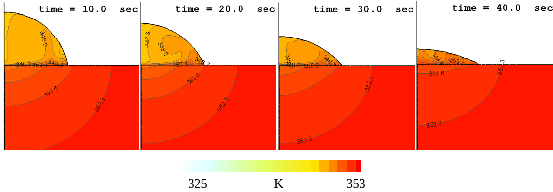
Figure 8: Predicted temperature distribution within the liquid and the solid during the vaporisation process using the full solution. [Initial surface temperature 80^{\circ}\text{C} , initial contact angle 90 degrees]
