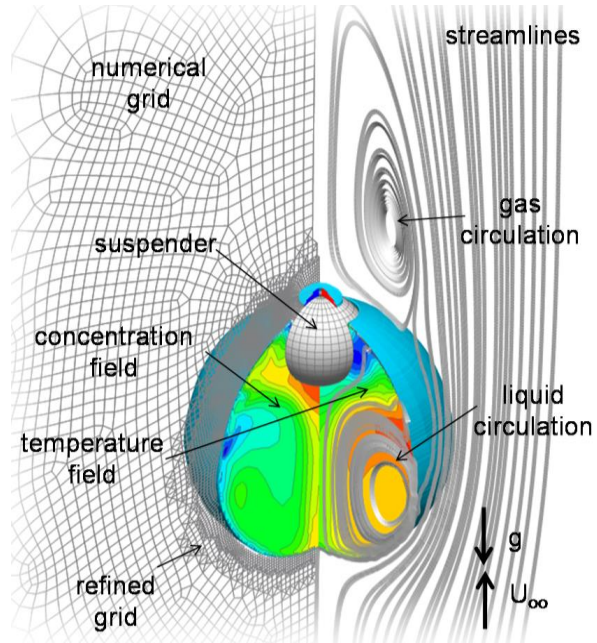
Fig. 1: A three-dimensional representation of one of the cases simulated. The numerical grid, selected streamlines, temperature and concentration fields inside the droplet are shown.
