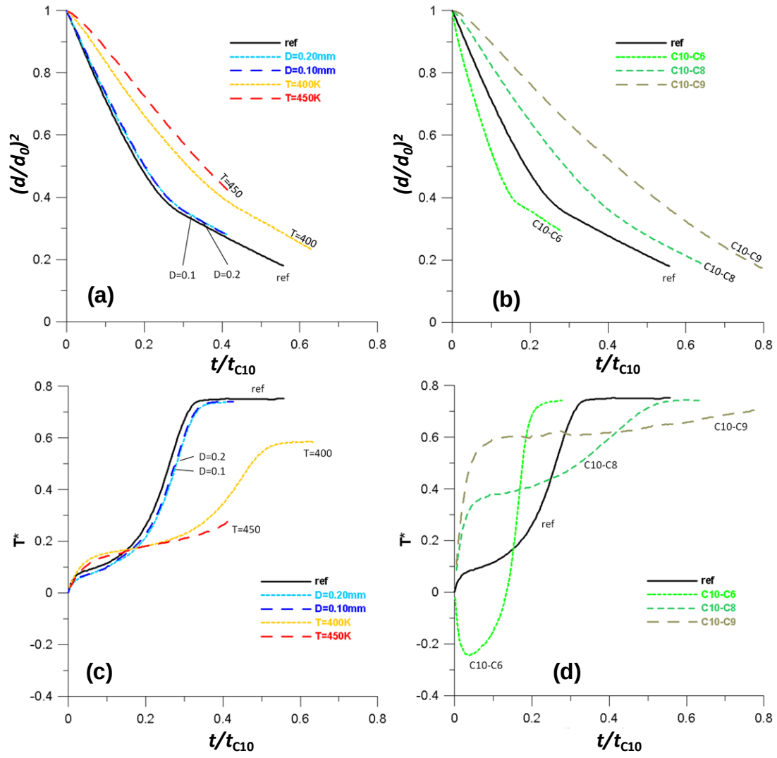
Fig. 17: Predicted temporal evolution of dimensionless droplet squared diameter (upper part a, b) and droplet's mean temperature (lower part c, d), showing the influence of the droplet size, gas phase temperature (left part a,c) and species volatility difference (right part b, d).
