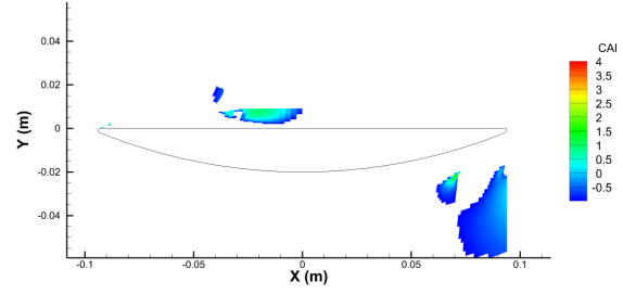
Figure 1f. CAI values on and around the hydrofoil.
