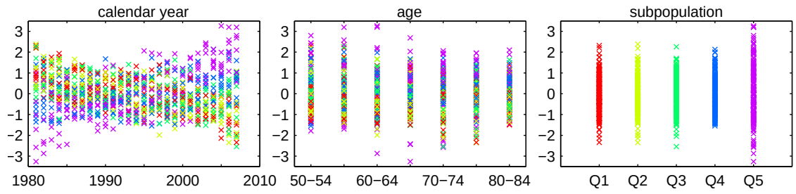
(C) Common factor: \log_n \mu_{xtg} = \alpha_x + \alpha_{xg} + \beta_x \kappa_t
