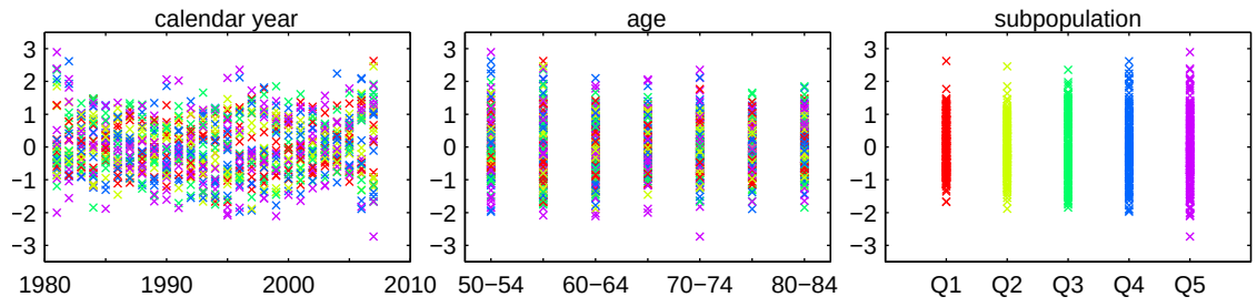
(A) Lee-Carter: \log_n \mu_{xtg} = \alpha_{xg} + \beta_{xg} \kappa_t
