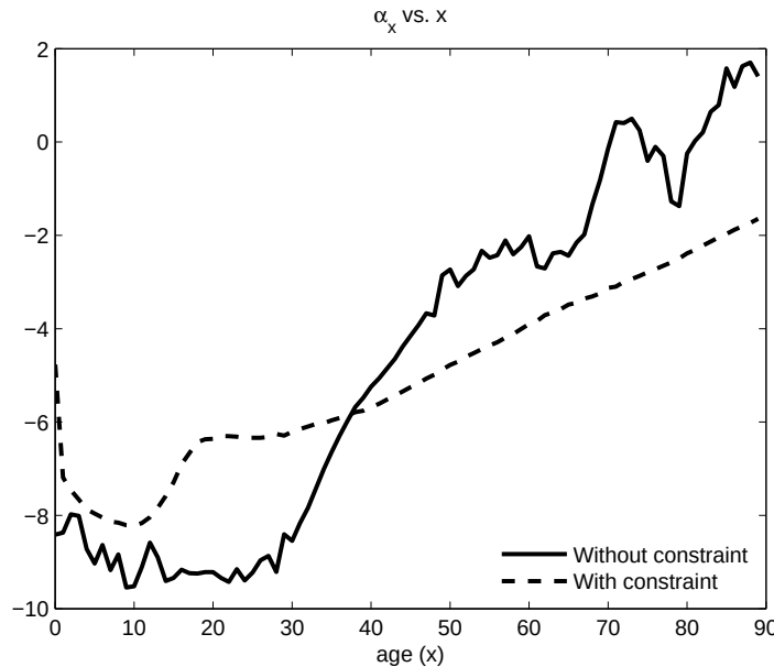
FIGURE 6.15: \alpha_x parameters for model M for for USA male data for ages 0-89 and period 1961-2007 fitted using the one-stage approach without and with the approximate identifiability constraint.
