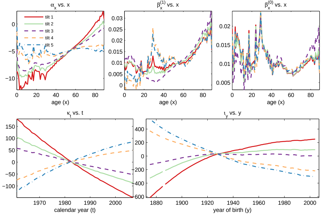
FIGURE 6.6: Parameters for model M with different initial parameters estimates fitted using the one-stage approach.
