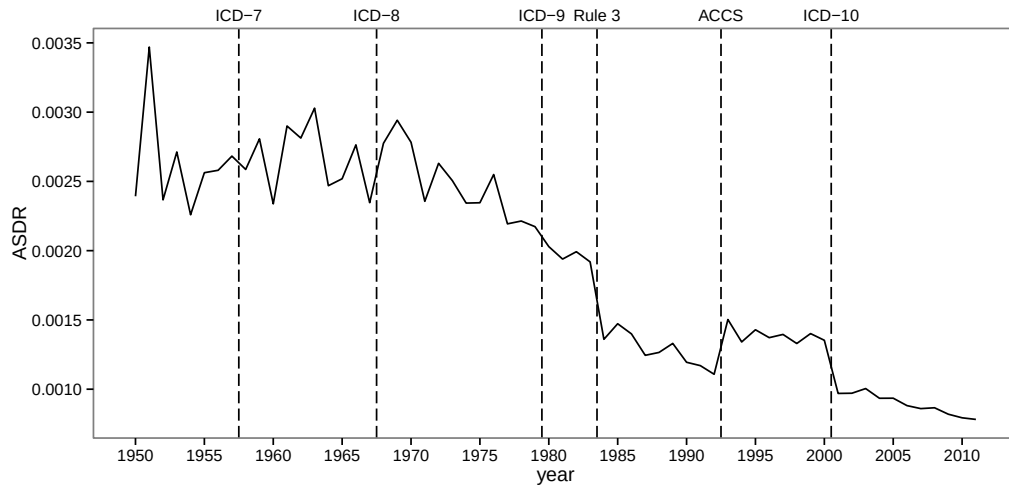
FIGURE 3.1: Age-standardised mortality rate for respiratory diseases for men aged 25-84 in England and Wales for the period 1950-2011.
