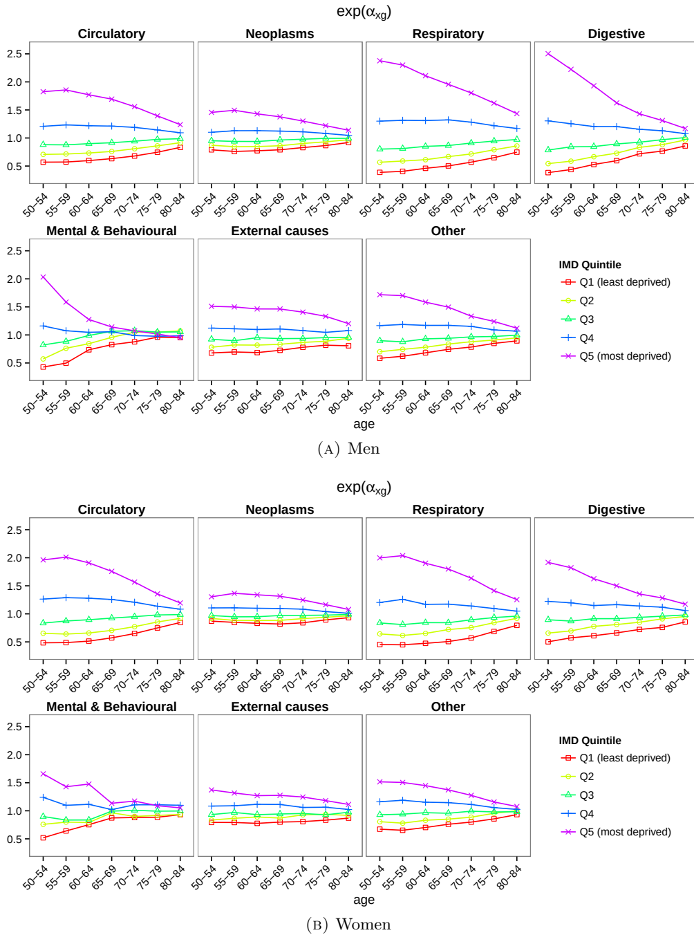
FIGURE 3.14: Mortality level differentials for the different causes of death across deprivation quintiles of England ( \exp(\alpha_{xg}) )
