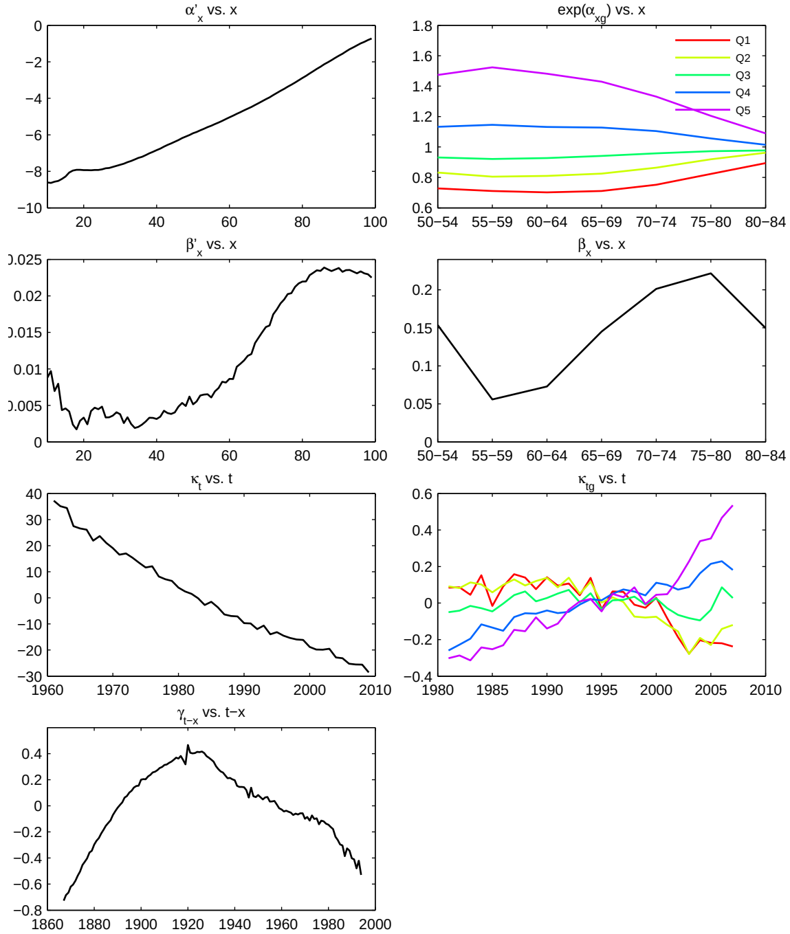
FIGURE 2.8: Parameter estimates of the relative model for the female deprivation subpopulations with age-period-cohort reference.
