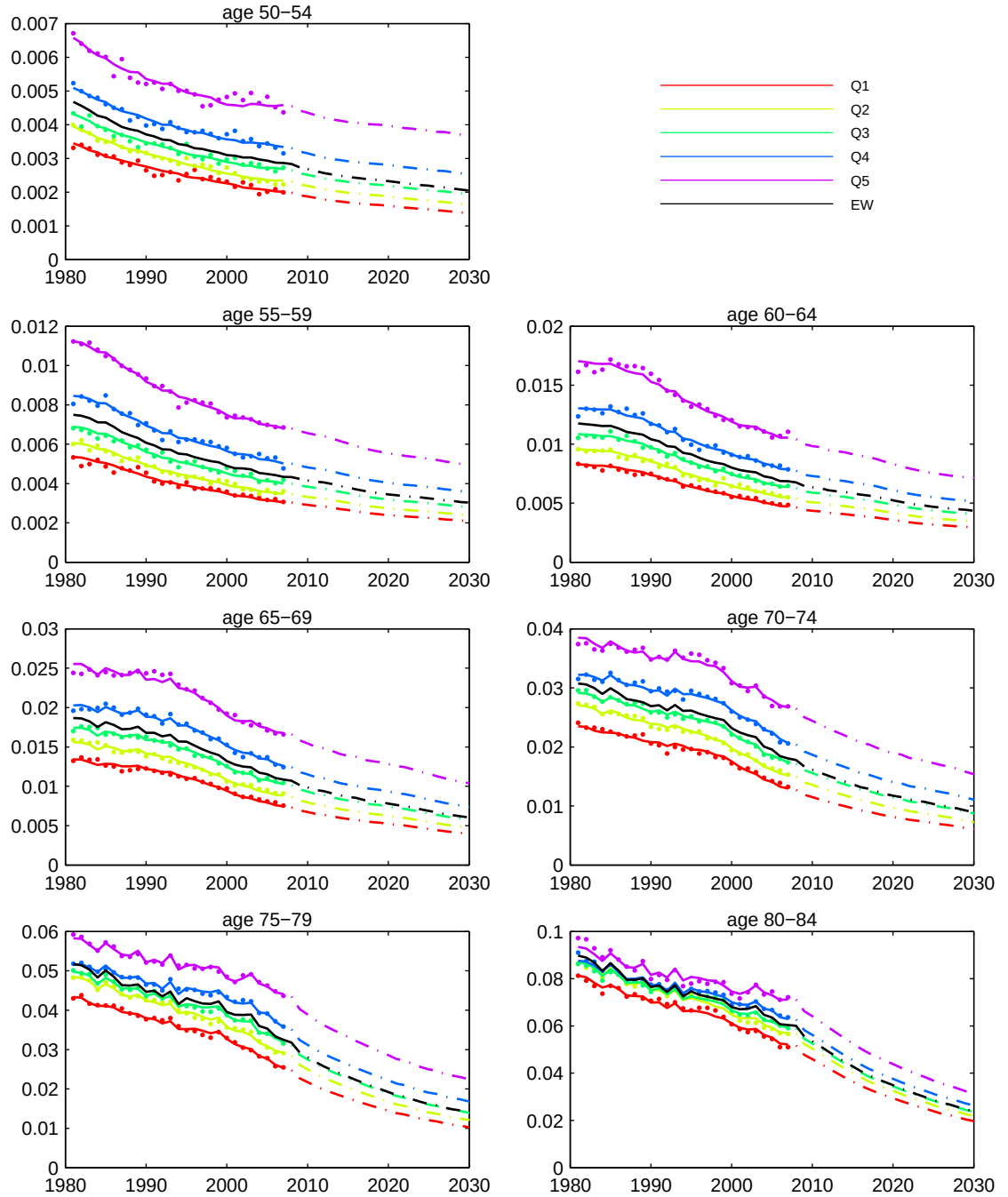
FIGURE 2.15: Time series of fitted and forecasted mortality rates {}_5\mu_{xtg} for the female deprivation subpopulations.
