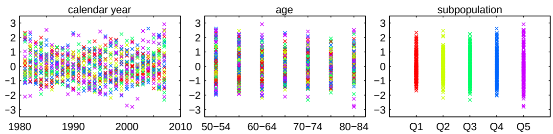
(E) Three way Lee-Carter: \log_n \mu_{xtg} = \alpha_x + \alpha_{xg} + \beta_x \lambda_g \kappa_t
