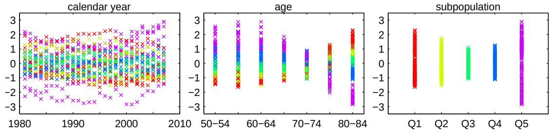
(B) Stratified Lee-Carter: \log_n \mu_{xtg} = \alpha_x + \alpha_g + \beta_x \kappa_t
