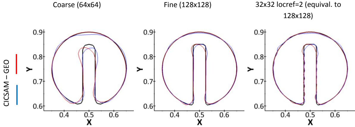
Figure 18. Use of Geo-Reconstruct in Benchmark case1, Zalesak’s disk. Comparison between Geo-Reconstruct and CICSAM.
