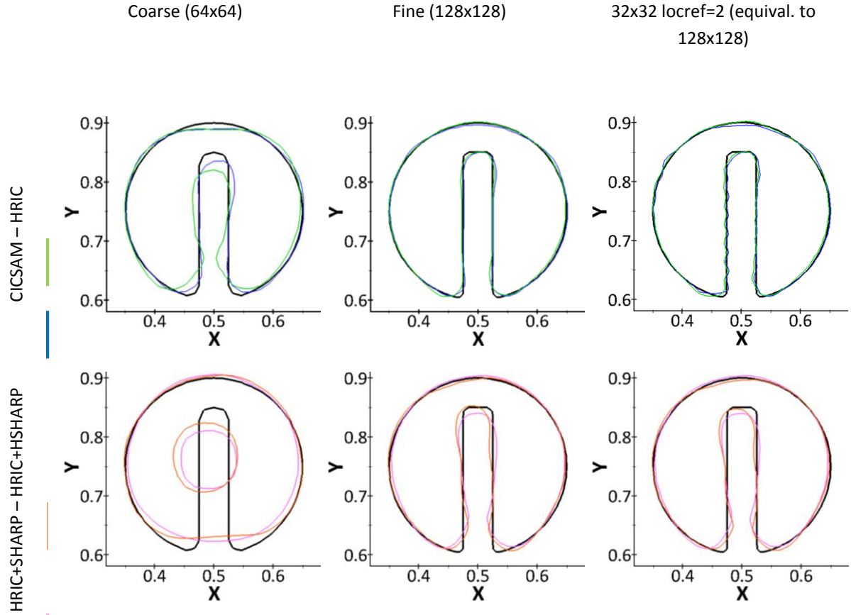
Figure 5. Zalesak's disk after one revolution. Isoline of \alpha=0.5 is plotted, together with the reference shape.
