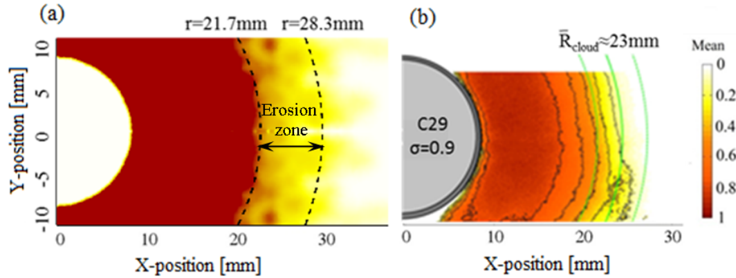
Fig. 11( \sigma=0.9 and P_{down}=19\text{bar} ) where the time averaged probability of vapour presence is shown for both the experiment and the hybrid RANS/LES results, projected on the lower disk; the probability was estimated based on a threshold value which was 5% vapour fraction for the CFD calculations (i.e. if the average vapour fraction at the line of sight is more than 5%, then the probability is 1, else it is zero). The comparison indicates similar locations of bubble cloud formation and collapse regions, e.g. the vapour structures begin to collapse at \sim 20\text{mm} from the axis of symmetry (see Fig. 10) and may disappear just after the 25\text{mm} . Regarding the vapour distribution in the normal direction between the two disks no experimental data are available. However, on average, the vapour distribution from the CFD results shows a stronger vapour presence near the upper disk and this could possibly correlate to the extended erosion zone found at the specific disk.
