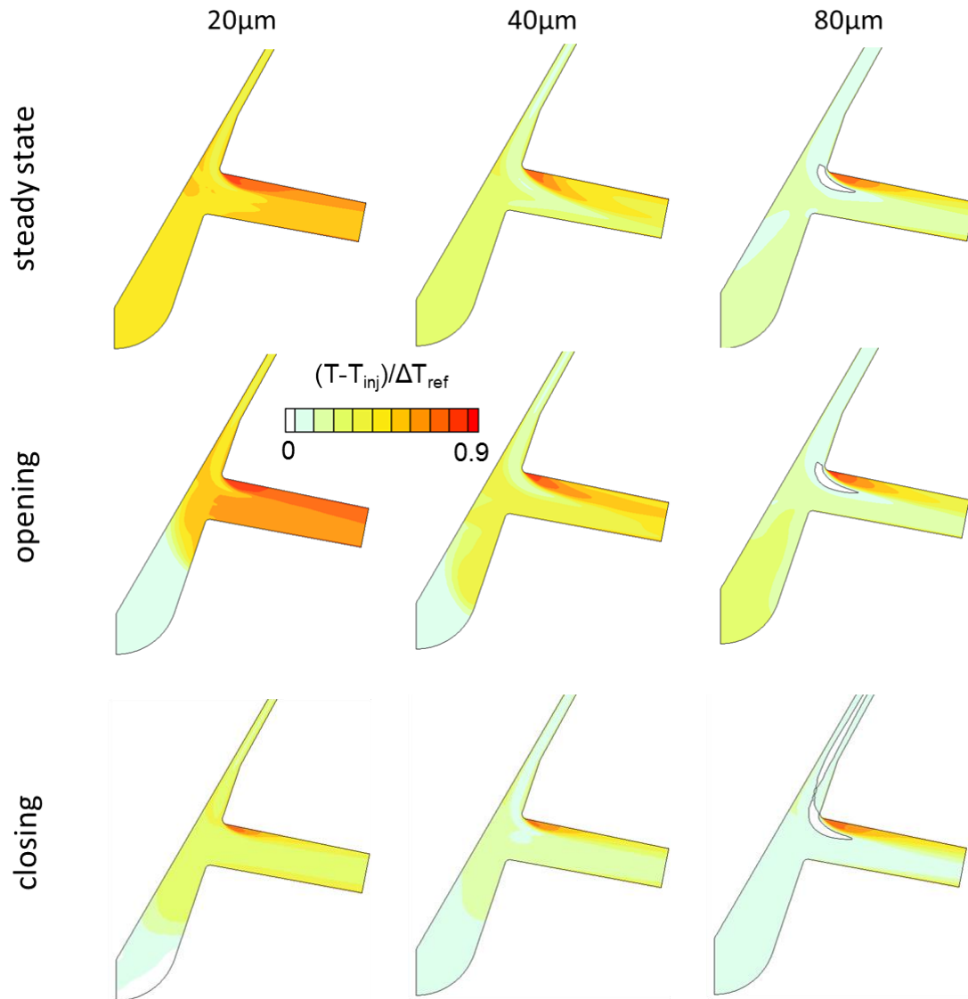
Fig.9: Temporal evolution of the dimensionless temperature field for the adiabatic nozzle. Comparison between the opening and the closing phases. Corresponding predictions from steady state simulations are also presented. 2000bar, single-phase, variable properties.
