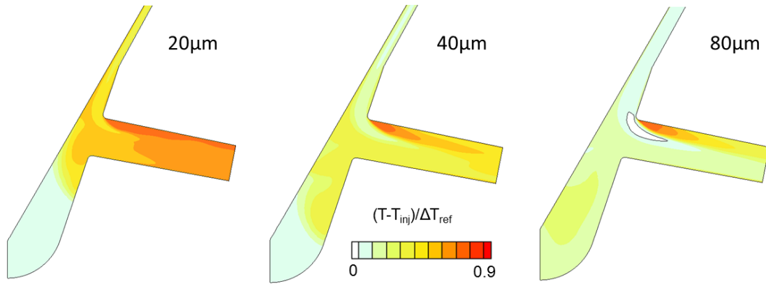
Fig.11: Temporal evolution of the dimensionless temperature field for the nozzle with constant surface temperature (80°C, opening phase).
