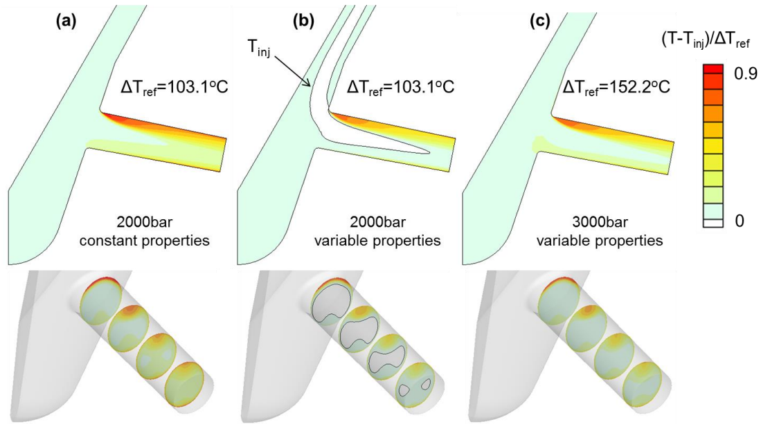
Fig.8: Dimensionless temperature field for the case of single phase flow at 200μm lift. (a) constant properties, 2000bar, (b) variable properties, 2000bar, (c) variable properties, 3000bar.
