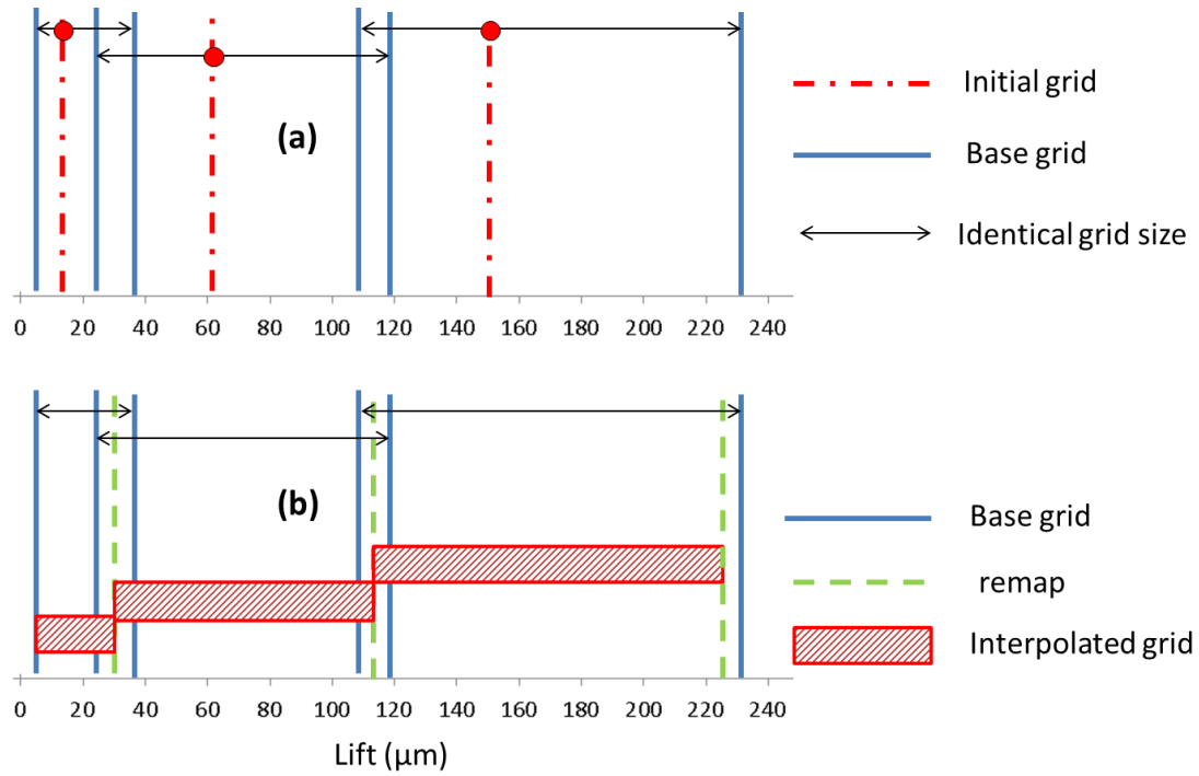
Fig.2: Computational technique for the grid adaption in moving lift.
