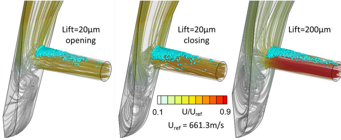
Fig.6: Dimensionless velocity field along with indicative cavitation bubbles for the case of two phase flow with 2000bar inlet pressure at 20μm lift (opening and closing phase) and 200μm.
