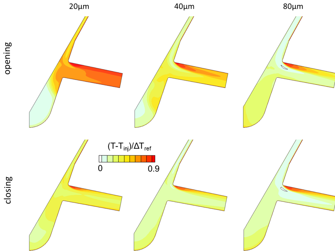
Fig.10: Temporal evolution of the dimensionless temperature field for the nozzle with constant surface temperature (300°C). Comparison between the opening and the closing phases for the case of 2000bar inlet pressure.
