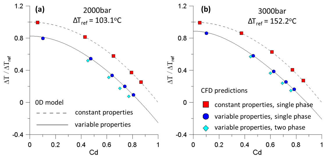
Fig.4: Dimensionless fuel heating for 2000bar (a) and 3000bar (b) inlet pressures. The effect of constant or variable properties assumption, as also the effect of two-phase flow is presented.
