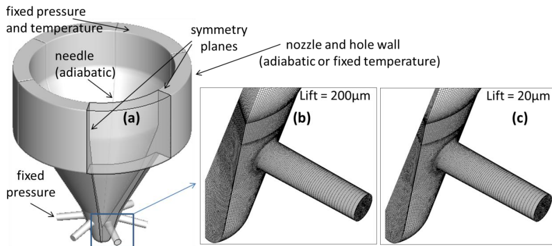
Fig.3: Nozzle geometry and grid details. (a)Computational domain and boundary conditions utilized, (b, c) Detail of the computational mesh at 200μm and 20μm needle lift respectively.
