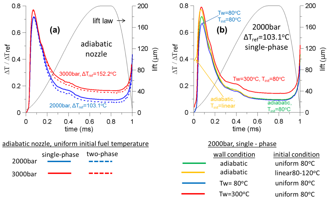
Fig.5: (a) Lift law and fuel heating versus time; solid lines refer to single-phase flow and dashed lines refer to two-phase flow. (b) Effect of initial and boundary conditions for fuel heating.
