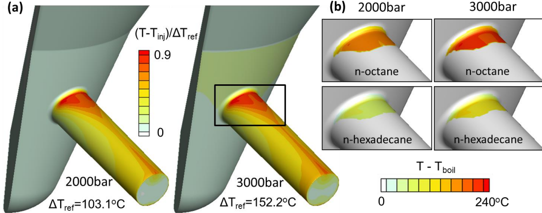
Fig.12: (a) Dimensionless surface temperature, (b) boiling overheat for a light and a heavy Diesel component. Two phase flow at 200 \mu\text{m} lift for the cases of 2000 and 3000bar inlet pressure.
