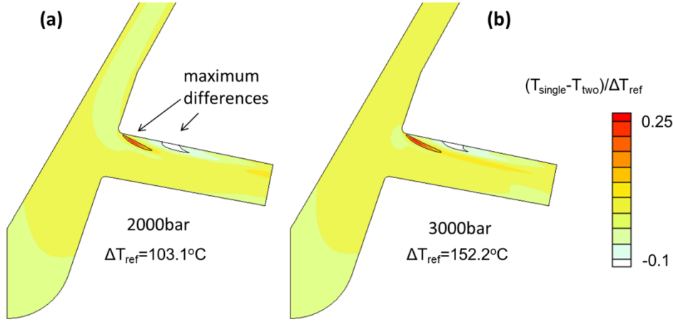
Fig.7: Dimensionless temperature difference between the single-phase and two-phase fields for the case of 200μm lift. (a) 2000bar inlet pressure, (b) 3000bar inlet pressure.
