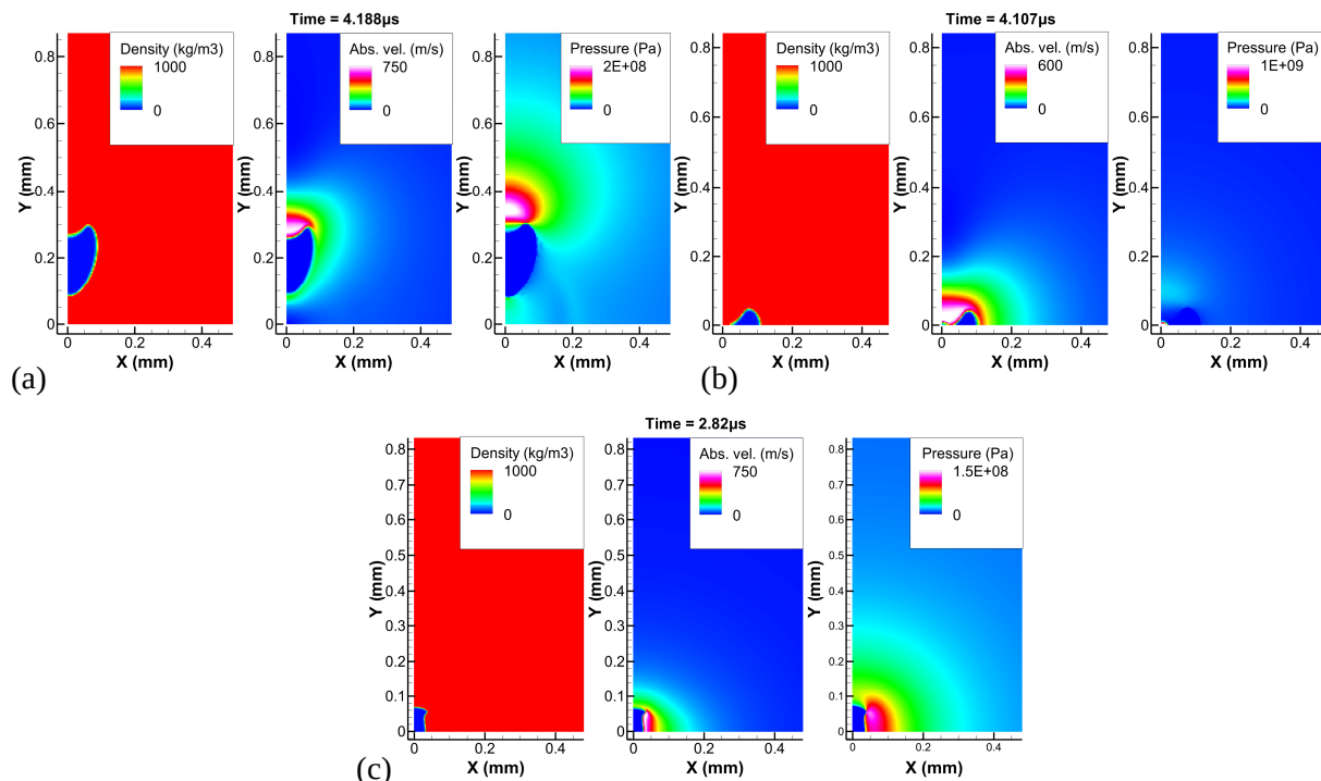
Fig. 2. Indicative instance from the collapse of a bubble placed (a) 416 \mu m (b) 140 \mu m and (c) -140 \mu m from a wall; y-axis is axis of symmetry, x-axis is wall.
