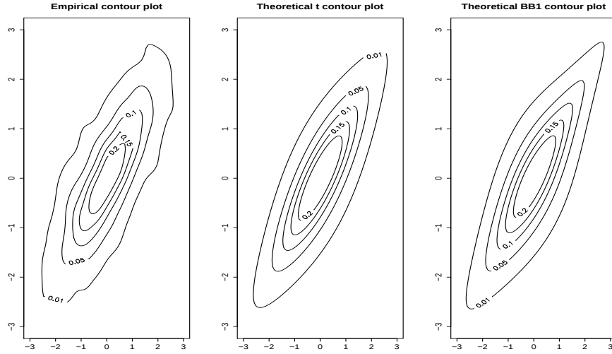
Figure 3.6.1: Empirical and theoretical contour plots for assessing the fit of Student- t and BB1 copulas on the transformed pair-copula F1BQ-F1BY Phelix Baseload data.
