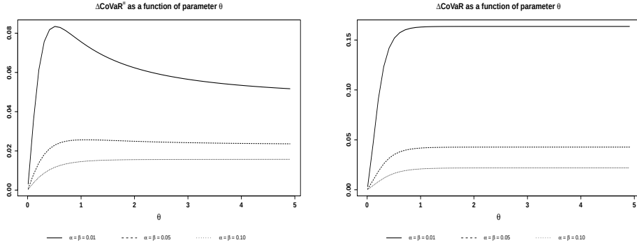
Figure 4.3.1: Clayton with Student- t margins with 3 degrees of freedom: \Delta CoVaR_{\alpha,\beta,t}^= and \Delta CoVaR_{\alpha,\beta,t} as a function of \theta .
