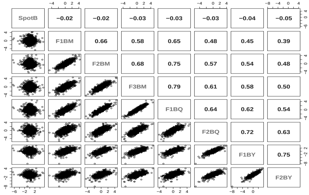
Figure 3.6.3: Dependence structure of standardised residuals in the Baseload portfolio. Upper diagonal matrix: Sample Kendall's \tau correlation coefficients for each pair of standardised residual series. Lower diagonal matrix: Bivariate scatter plots for each pair of standardised residual series.
