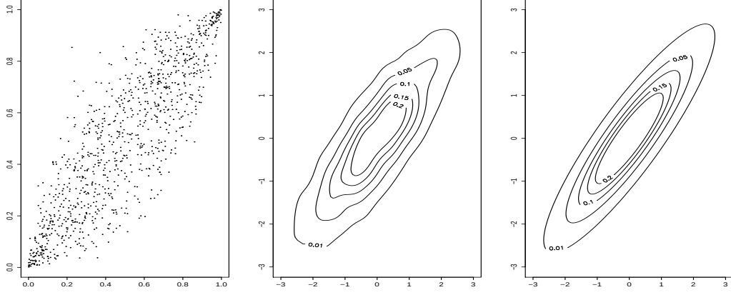
(a) Scatter plot, theoretical and empirical contour plots of a Normal copula with dependence parameter \tau = 0.7 , \rho = 0.8910065 and \lambda_L = \lambda_U = 0 .
