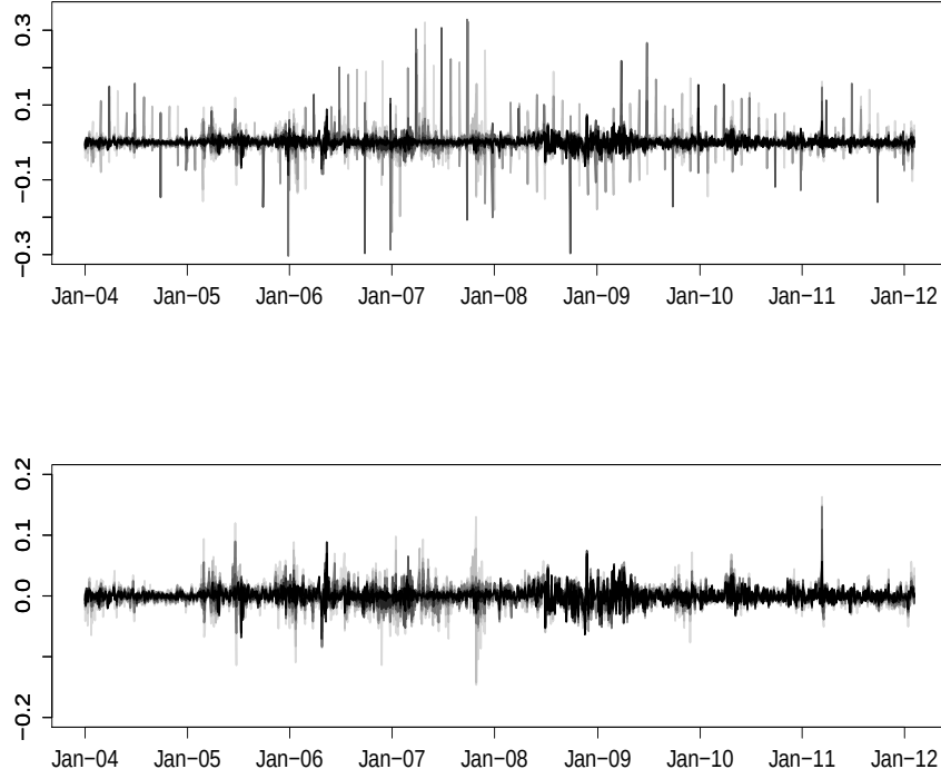
Figure 3.5.1: Upper: Log-returns of generic Phelix Baseload futures without adjustment for the roll-over of futures contracts. Lower: Log-returns of generic Phelix Baseload futures with adjustment for the roll-over of the futures contracts.
