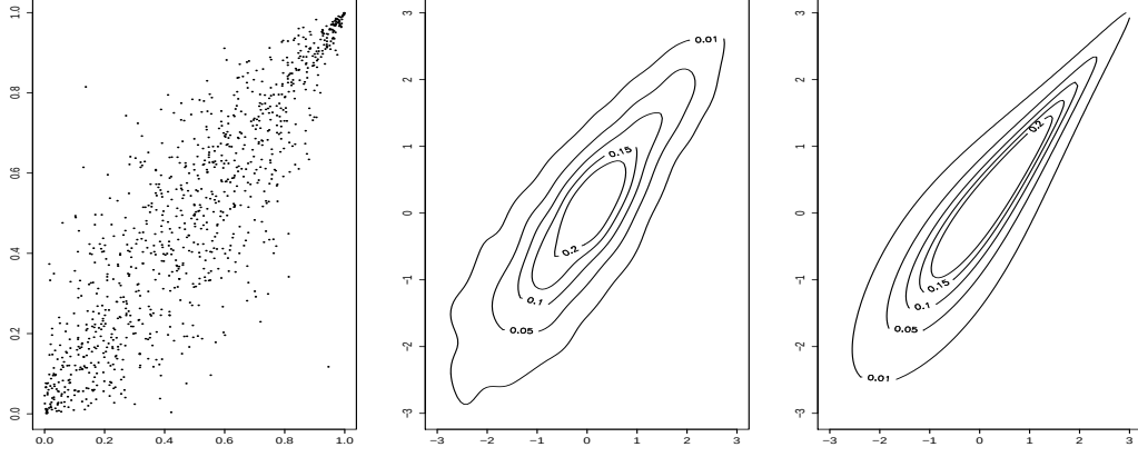
(a) Scatter plot, theoretical and empirical contour plots of a Gumbel copula with dependence parameter \tau = 0.7 , \hat{\theta} = 3.333333 , \lambda_L = 0 and \lambda_U = 0.7688556 .
