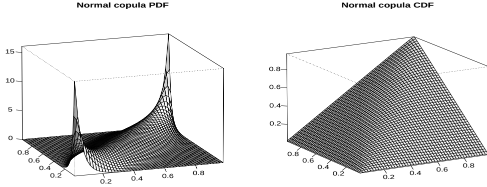
(a) CDF and PDF of a bivariate Normal copula with dependence parameter \tau = 0.7 , \rho = 0.8910065 and \lambda_L = \lambda_U = 0 .
