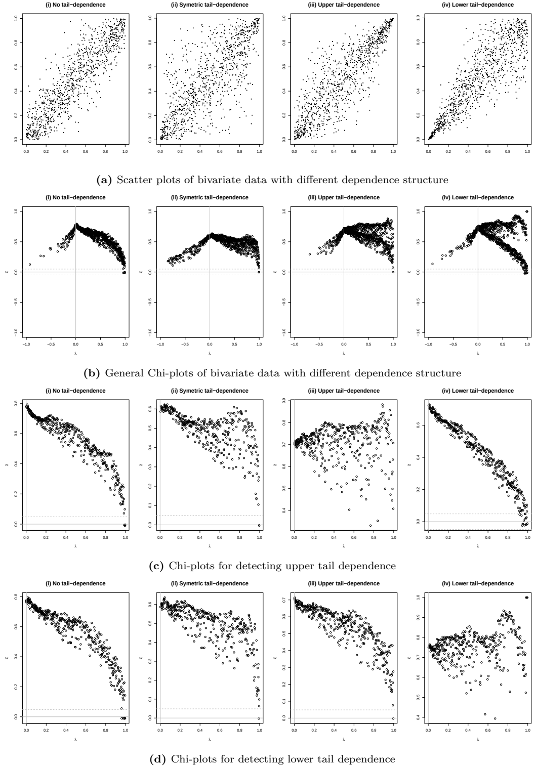
Figure 2.10.3: Chi-plots for detecting (tail) dependence: (a) bivariate scatter plots with different dependence form; (b) General Chi-plots; (c) Chi-plots for upper tail dependence; (d) Chi-plots for lower tail dependence.
