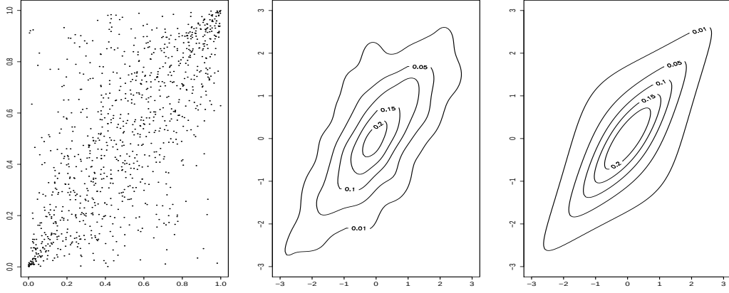
(b) Scatter plot, theoretical and empirical contour plots of a Student- t copula with dependence parameter \tau = 0.7 , 3 degrees of freedom and \lambda_L = \lambda_U = 0.4480999 .
