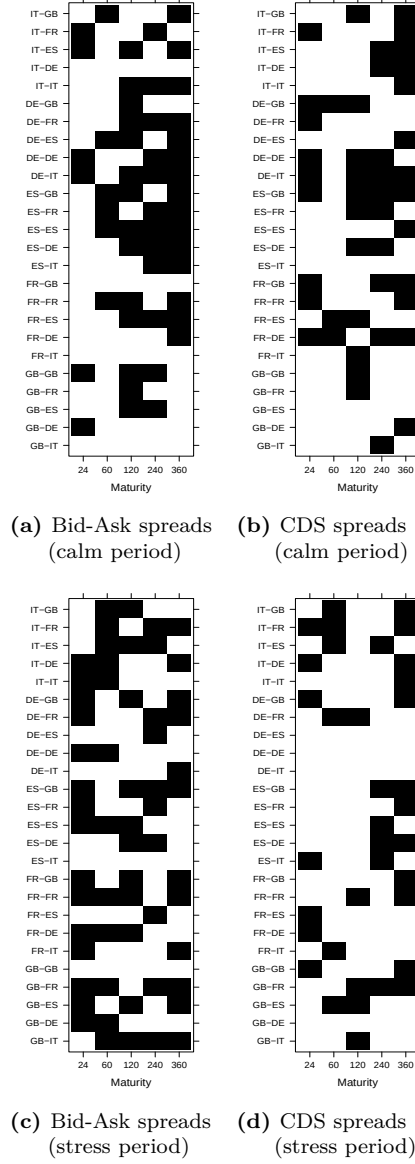
Figure 5.7.3: This figure demonstrates the significance of the estimated coefficients, at selected maturities, from the covariance regression model in calm and stress periods. White cells indicate significance at 5% level, while Black cells indicate insignificance of the estimated coefficient at 5% level. Figure 5.7.3a presents the significance of country-specific liquidity measures (bid-ask spreads), whereas Figure 5.7.3b presents the significance of country-specific credit measures (credit default swap (CDS) spreads) in explaining the covariation for each individual pair of countries in the calm period. Figure 5.7.3c presents the significance of country-specific liquidity measures (bid-ask spreads), whereas Figure 5.7.3d presents the significance of country-specific credit measures (credit default swap (CDS) spreads) in explaining the covariation for each individual pair of countries in the stress period. The first country of each pair represents the row, while the second country represents the column of matrix \mathbf{B} in Equation (5.12). In addition, the second country indicates the origin of the country-specific explanatory variable in the covariance regression model.
