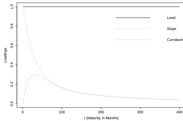
Figure 5.4.1: Factor loadings of the Nelson-Siegel model with fixed \lambda = 0.0609 .
