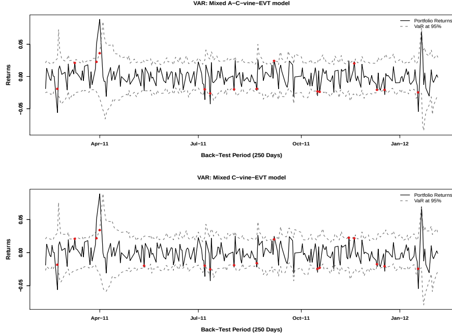
Figure 3.7.1: Baseload portfolio returns and 95%- VaR forecasts for the A-C-vine-EVT and C-vine-EVT models. VaR exceedances are marked by red points
