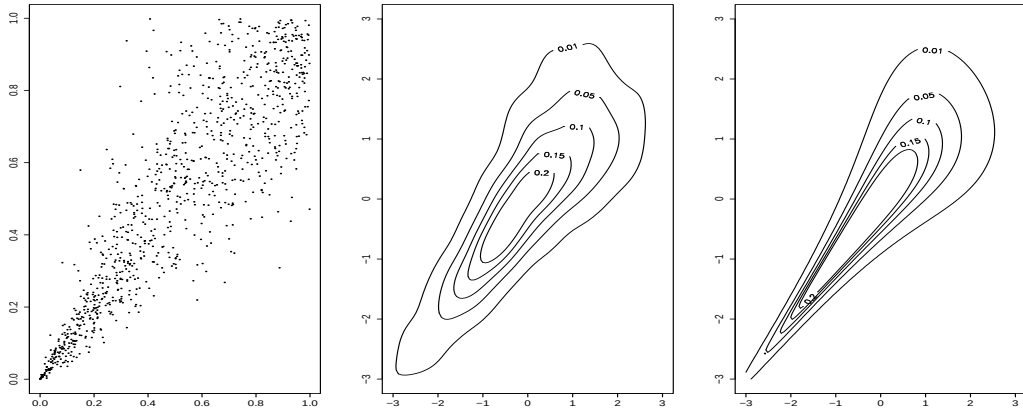
(c) Scatter plot, theoretical and empirical contour plots of a Clayton copula with dependence parameter \tau = 0.7 , \hat{\theta} = 4.666667 , \lambda_L = 0.8619728 and \lambda_U = 0 .
