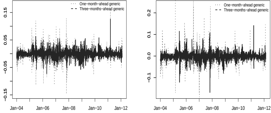
Figure 3.5.2: Left: Log-returns of generic Phelix Baseload one-month-ahead and three-months-ahead power futures. Right: Log-returns of generic Phelix Peakload one-month-ahead and three-months-ahead power futures.
