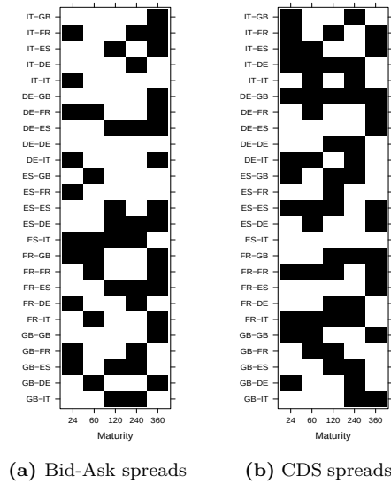
Figure 5.7.2: This figure demonstrates the direction of the estimated coefficients, at selected maturities, from the covariance regression model. The white cells indicate negatively-signed estimated coefficients, while the black cells indicate positively-signed estimated coefficients. Figure 5.7.2a presents the signs of the country-specific liquidity measures (bid-ask spreads) whereas Figure 5.7.2b presents the signs of the country-specific credit measures (credit default swap (CDS) spreads). The first country in each pair represents the row, while the second country represents the column of matrix B in Equation (5.12). In addition, the second country indicates the origin of the country-specific explanatory variable in the covariance regression model.
