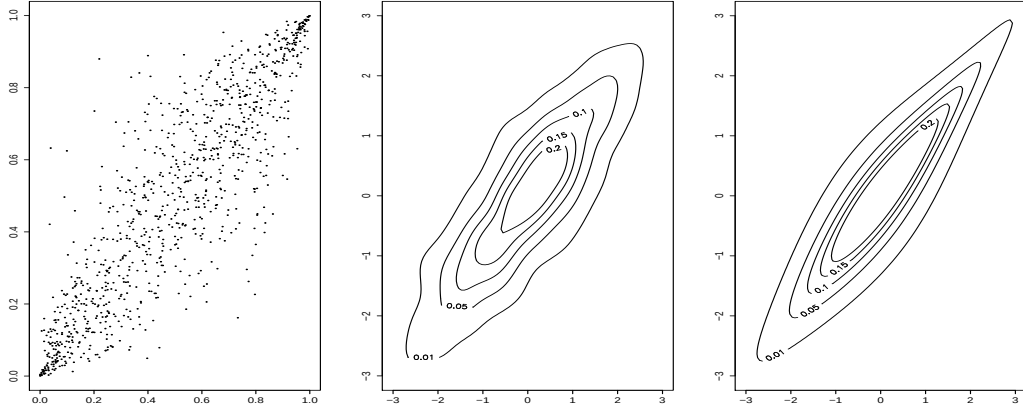
(b) Scatter plot, theoretical and empirical contour plots of a BB1 copula with dependence parameter \hat{\tau} = 0.7007108 , \theta = 0.43 , \delta = 2.75 , \lambda_L = 0.5564539 and \lambda_U = 0.7133351 .
