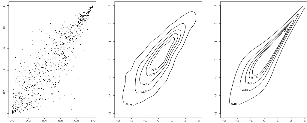
(c) Scatter plot, theoretical and empirical contour plots of a BB7 copula with dependence parameter \hat{\tau} = 0.7001527 , \theta = 4.8 , \delta = 0.82 , \lambda_L = 0.4294279 and \lambda_U = 0.8446473 .
