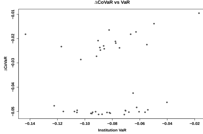
Figure 4.6.3: This scatter plot shows the cross-sectional link between the time-series average of each financial institution's risk in isolation, measured by Var_{\alpha,t}^i , and the time-series average contribution to systemic risk, measured by \Delta CoVaR_{\alpha,\beta,t} . All risk measures are generated under the assumption of Skewed- t margins and computed at \alpha = \beta = 5\% level.
