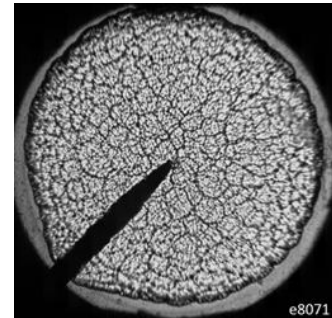
(c) p = 4.0 bar, ϕ = 1.4
