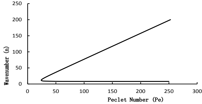
Fig. 2.1: Graph of cell wavenumber (n) versus Peclet number (Pe) for p = 2.0 bar, ϕ = 1.4 flame.
