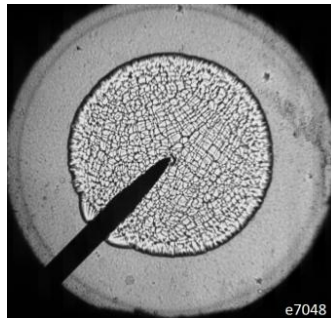
(b) p = 3.0 bar, ϕ = 1.4
