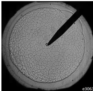
Figure 3.1(a) p = 2.0 bar, ϕ = 1.4
