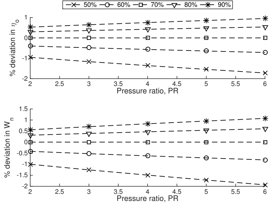
Figure 3.3: Sensitivity of the cycle performance to variations in the pump efficiency.
