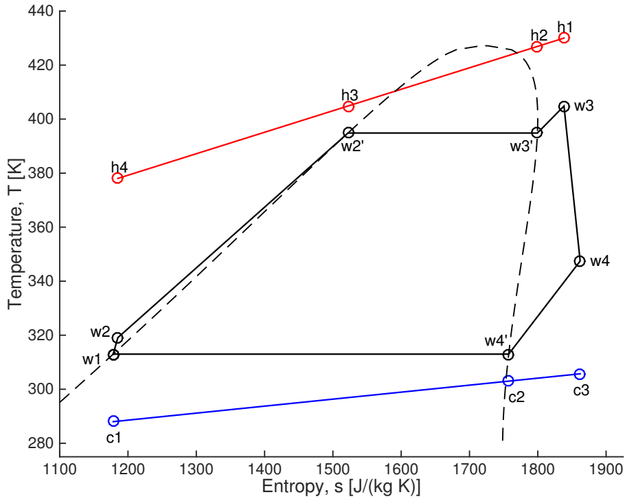
Figure 3.2: The subcritical, superheated ORC represented on a T-s diagram along with the heat source and heat sink temperature profiles, and the designated notation.
