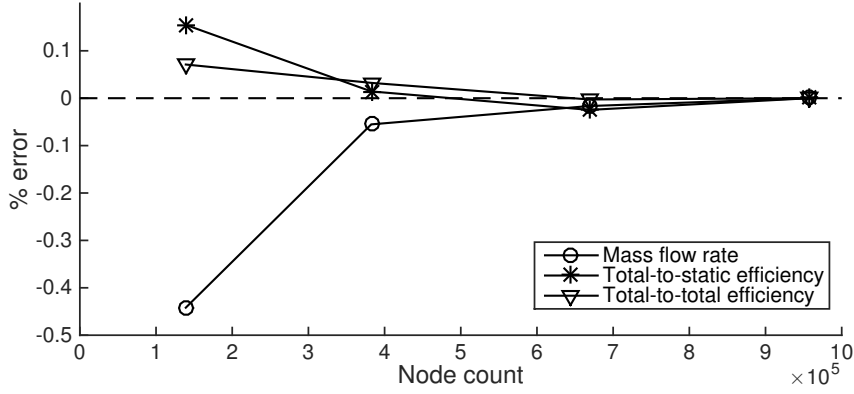
Figure 4.14: Grid independence study for the ORC turbine rotor with clearance gap.
