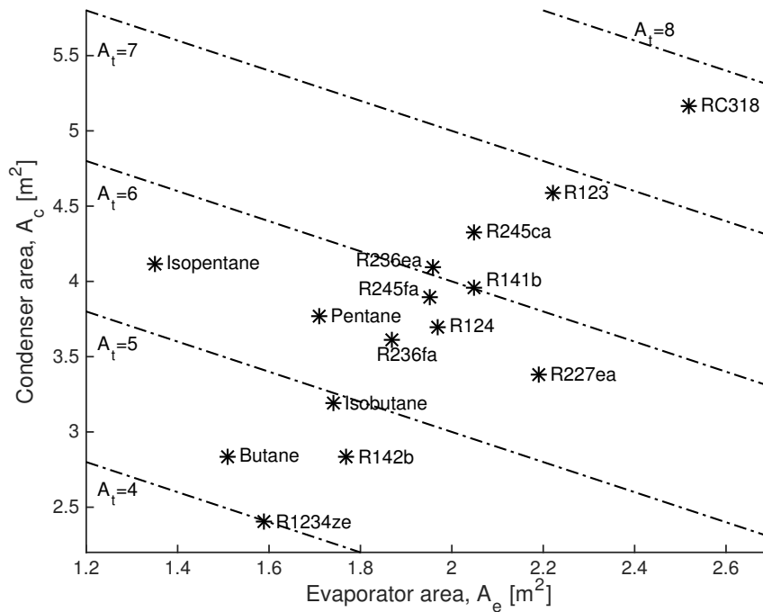
Figure 3.16: Evaporator and condenser areas that resulted from the sizing optimisation for the 15 working fluids considered.
