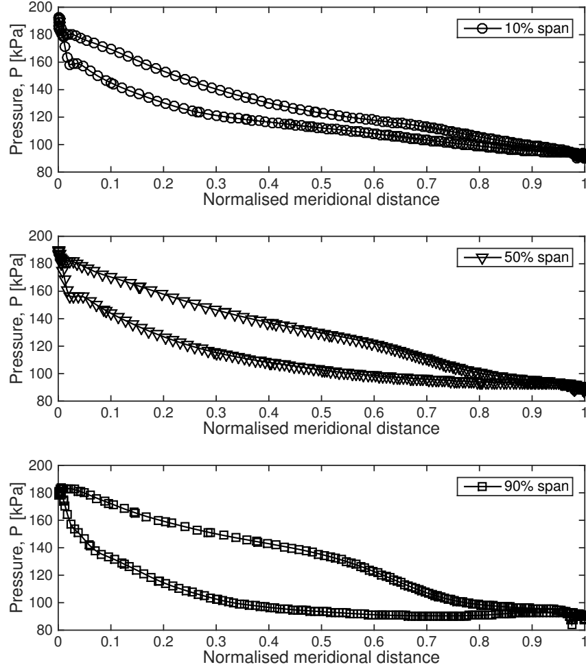
Figure C.4: Air blade loading at 10%, 50% and 90% span.
