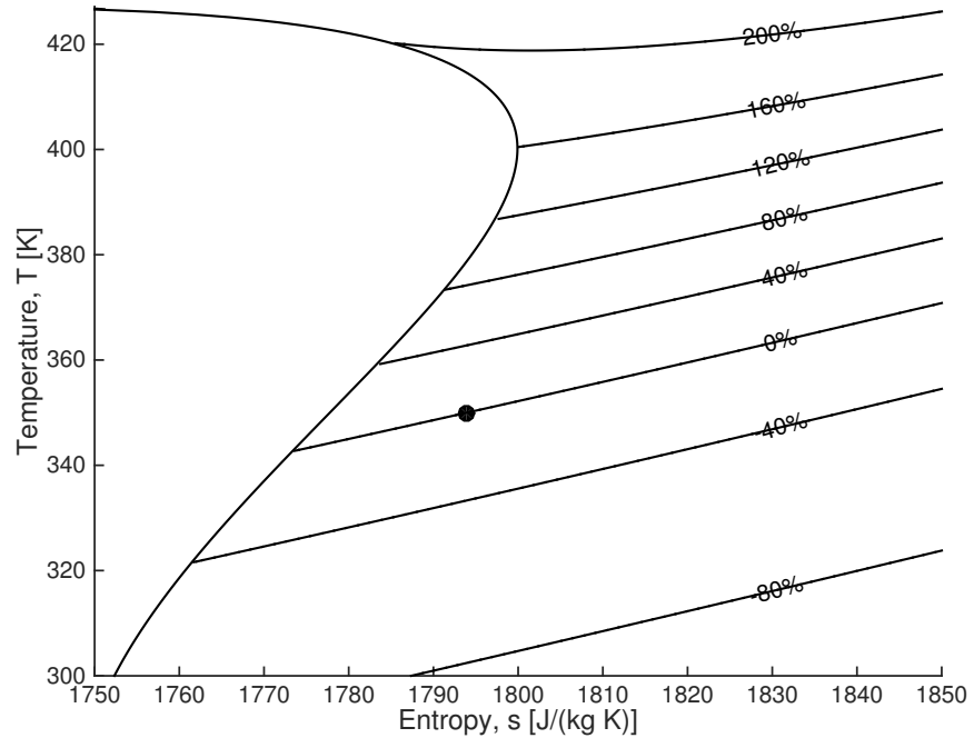
Figure 5.1: Deviation in Reynolds number with variations in turbine total inlet conditions for R245fa assuming that the blade Mach number has been conserved.
