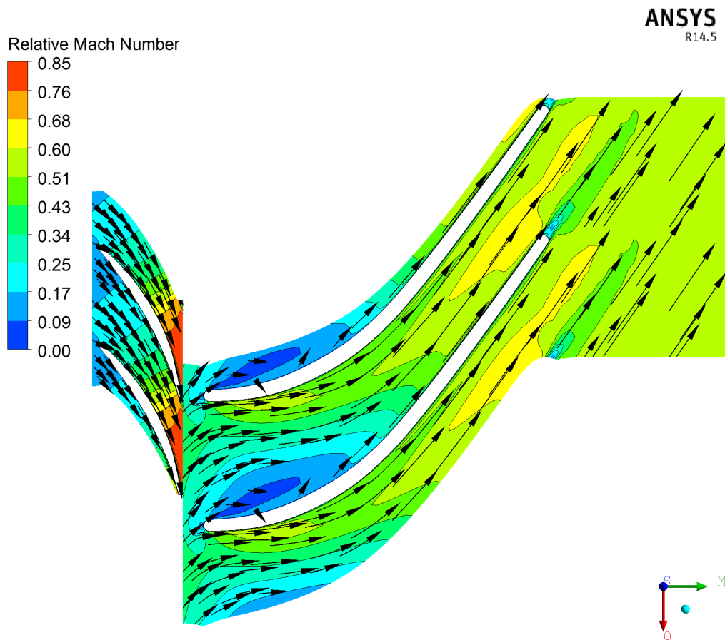
Figure C.5: Contour of relative Mach number and relative velocity vectors on the midspan of the air turbine.
