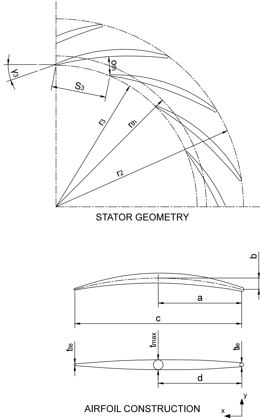
Figure 4.2: Schematic of the stator geometry and airfoil definition.
