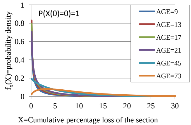
Figure 3 Gamma process representation following the inspection at year 13.
