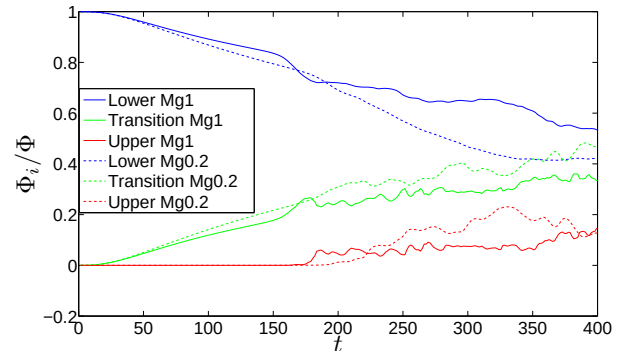
Figure 9. Temporal evolution of the magnetic flux fraction contained within the lower layer \Phi_L/\Phi , the transition region \Phi_T/\Phi and the upper layer \Phi_U/\Phi , in a simulation with M_\gamma = 1 (solid lines) and M_\gamma = 0.2 (dashed lines).
