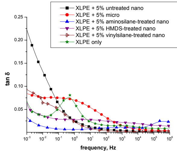
Figure 2. Dielectric spectroscopy of functionalized XLPE at 23 °C
