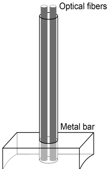
Fig. 2. Compression bar with optical fibers inserted.
