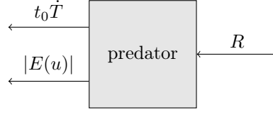
Figure 4.7: The evolutionary model of predator-prey interactions including elements of the predator lifetime model. The predator has an metabolic cost t_0\dot{T} and a behavioural expenditure |E(u)| . The costs are balanced by the influx of some fitness related quantity R .
