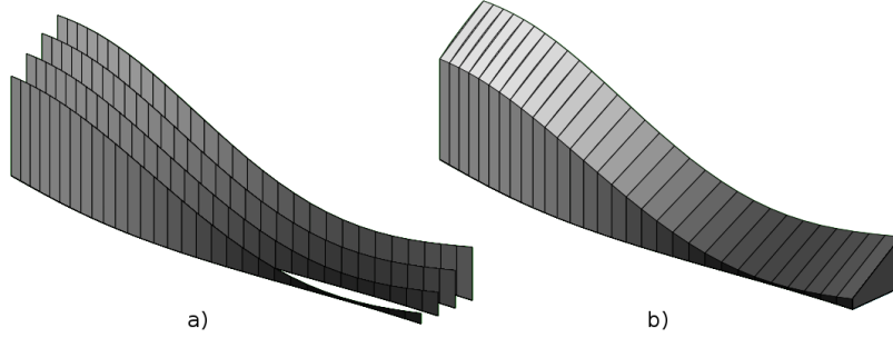
Figure 4.4: The reduction of necessary exploration when using b) VGL over a) BPTT. The VGL algorithm learns a wider range of the state space than the BPTT algorithm as the VGL weight update contains more information about adjacent trajectories. Figure by M. Fairbank taken from Fairbank (2013).
