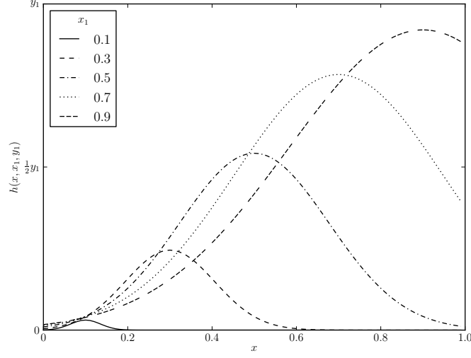
(a) This chart shows the generalisation of aversive information from an encounter with a specific morph (x_1, y_1) through the inhibitory gradient h(x, x_1, y_1) .
