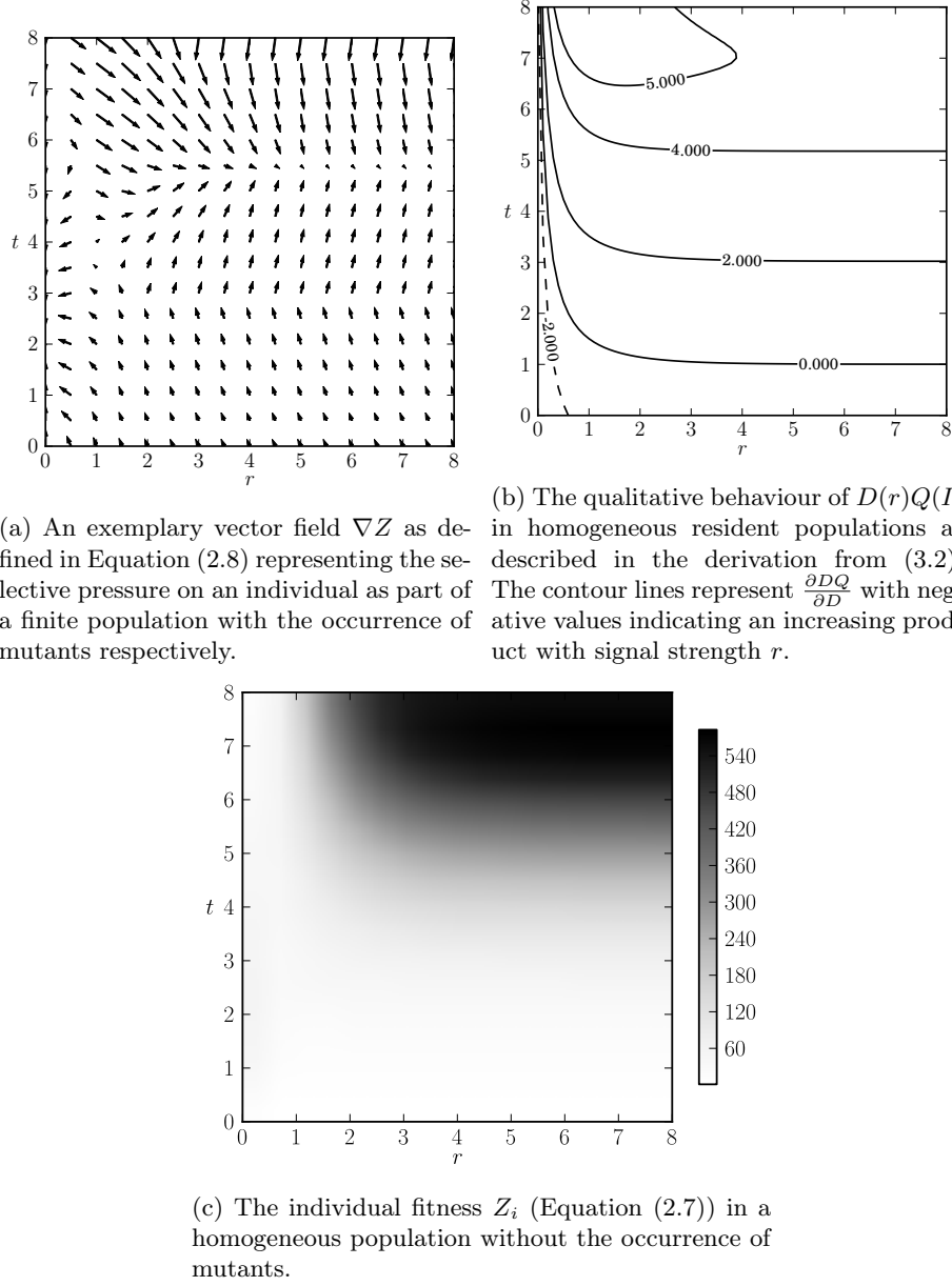
Figure 2.1: The different elements of evolutionary dynamics in the co-evolution of aposematism in finite populations. All parameters as in Figure 2.4a.
