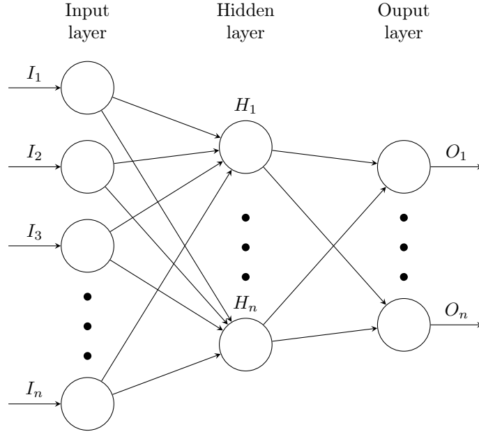
Figure 4.3: A feed-forward artificial neural network characterized by its distinctive layers.
