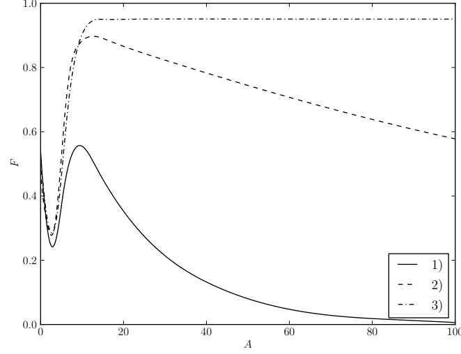
(a) This chart shows the variety of aposematic solutions as a result of the marginal cost of display \psi . 1) \psi = 1 , 2) \psi = 0.1 , and 3) \psi = 0 . All other parameters as in Speed and Ruxton (2007).
