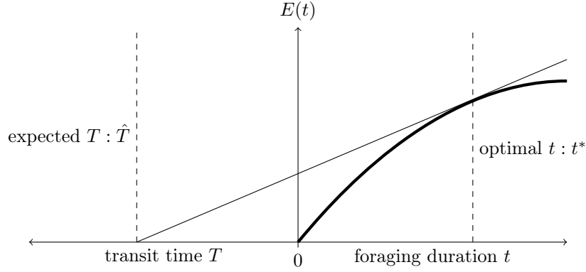
Figure 3.4: Marginal Value Theorem. The optimal foraging time in a patch t^* is given by the tangent of the cumulative energy gain from foraging in a patch E(t) .
