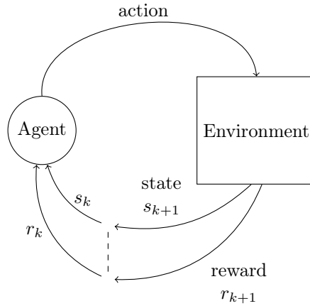
Figure 3.2: The reinforcement learning model with the two entities agent and environment. The agent's actions at iteration k have subsequent effects on the environment's state and rewards at iteration k + 1 . The dashed line indicates that the agent experiences the consequences of its actions with a delay.
