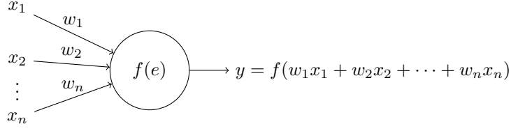
Figure 4.2: An abstract neuron representing a node in an artificial neural network. The neuron is evaluating its primitive function f(e) whereas the neurons excitement e is given by the weighted w inputs x .
