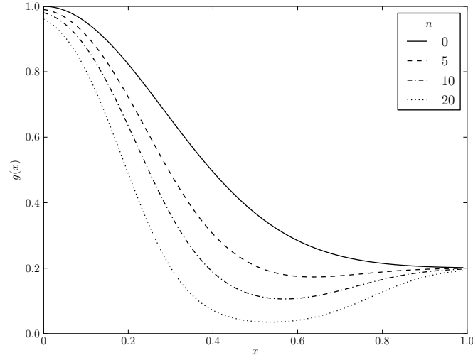
(b) This chart shows the attack probability g(x) after n encounters with prey of morph x_1 = 0.5 and y_1 = 0.2 . The graph for n = 0 shows the excitatory gradient e(x) of a naive predator. The graph for n > 0 show the peak-shift resulting in a bias towards the avoidance of more conspicuous prey.
