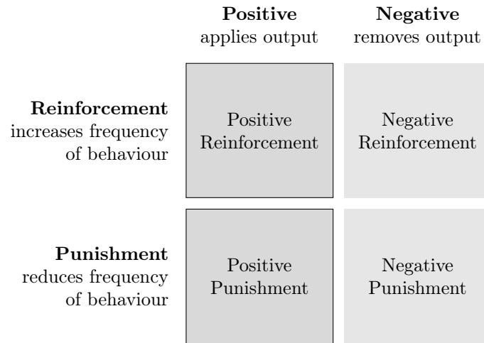
Figure 3.1: The different procedures in operant conditioning (or associative learning of actions and consequences) (Bouton, 2007).
