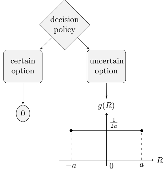
(a) The two options of the environment with the certain option being equal to zero and the uncertain option following a Uniform fitness payoff distribution g(R) with limits -a and a as given by Equation (3.20).
