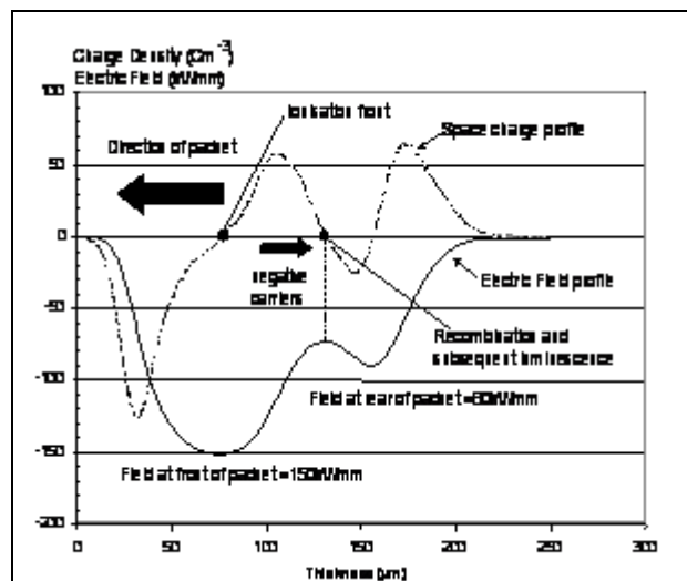
Figure 1: Charge packet in XLPE interpreted as a propagating ionization front and associated recombination-induced luminescence. The horizontal axis is distance through the material. The two curves correspond to space charge density (the positive "hump" is the charge packet) and the field (bottom curve). Cathode on the left, anode on the right. Taken from [7].
