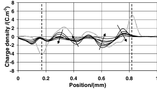
Figure 8: 10% \text{TiO}_2 nano-filled charge decay. Measurements made at 0 (volts on – grey curve), 10, 30, 60, 120, 300, 600, 900 and 1800 s.
