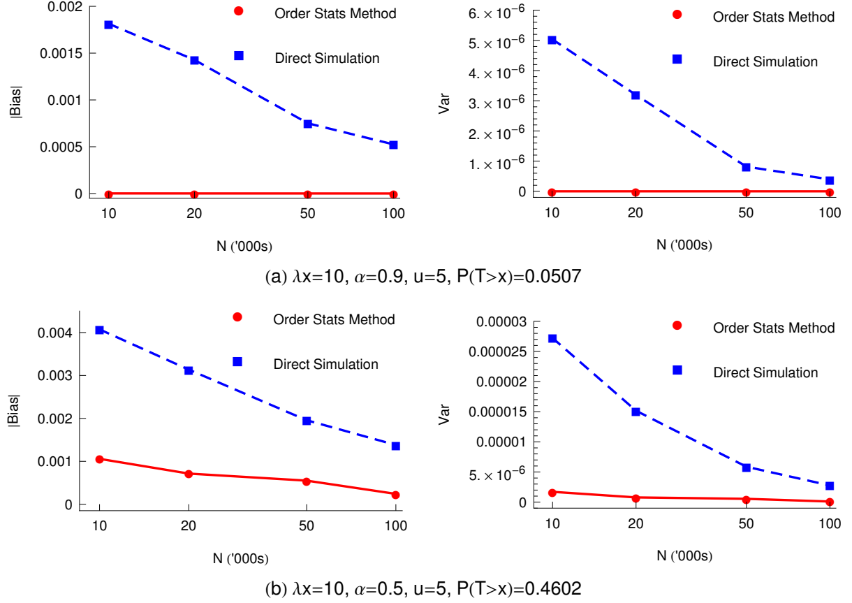
Figure 2: The absolute bias of the simulated estimates of P(T > x) (left panels) and their corresponding variances (right panels) using both the order statistics simulation-based method (red solid line) and direct MC simulation (blue dashed line), obtained with the assumptions of Example 6.1. Parameter values: \lambda = 1 , c = 1 , \epsilon = 10^{-4} , l_\epsilon^* = 0 , m_\epsilon^* = 15 ( n = 15 ) and M = 100 .
