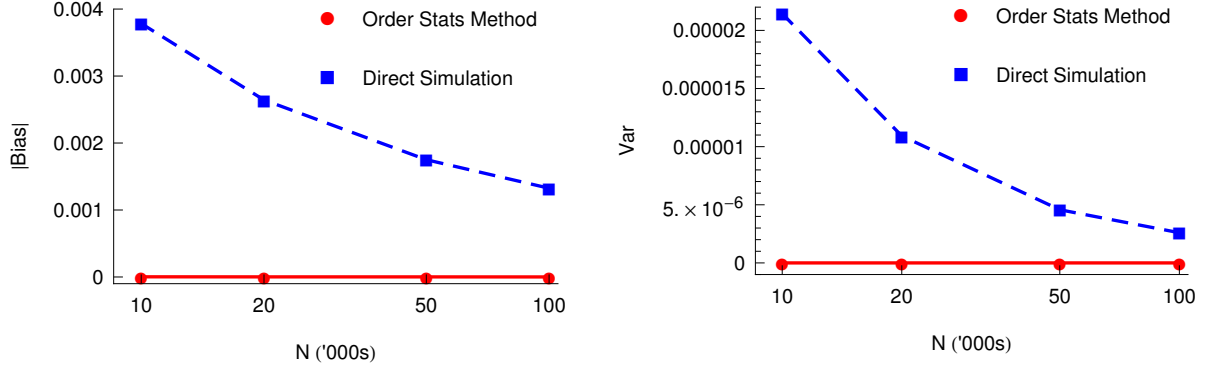
(a) \lambda x=5, \alpha=0.9, u=15, P(T>x)=0.5744
