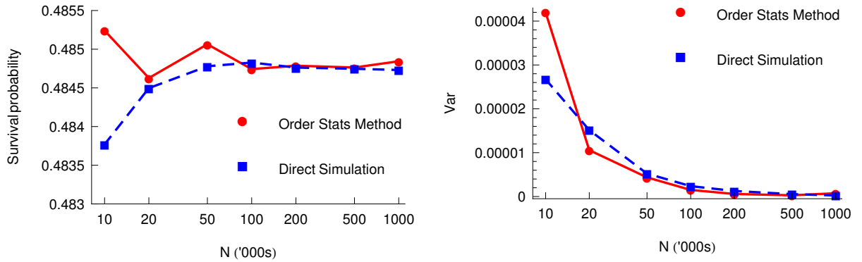
(b) \lambda x=5, \alpha_p=4, \lambda_p=2, \theta=1, u=5
