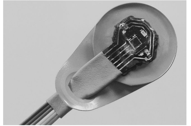
Fig. 2. Finished fontanel probe mounted onto an ECG electrode plastic base, and terminated with flat ribbon cable.
