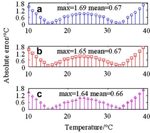
Fig. 5. Calibration measurement based absolute error values for the WB configuration. a) Channel used for environment temperature measurement in the T-history implementation. b) Channel used for PCM temperature measurement. c) Channel used for water temperature measurement.
