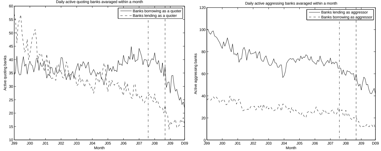
FIG. 10. Left: monthly average of the daily active banks acting as quoters. Right: monthly average of daily active banks acting as aggressors. In both cases the trades as been divided respecting the Sell and Buy label in the records, indicating that the money are flowing from the aggressor to the quoter in the first case, and in the opposite way in the second case.
