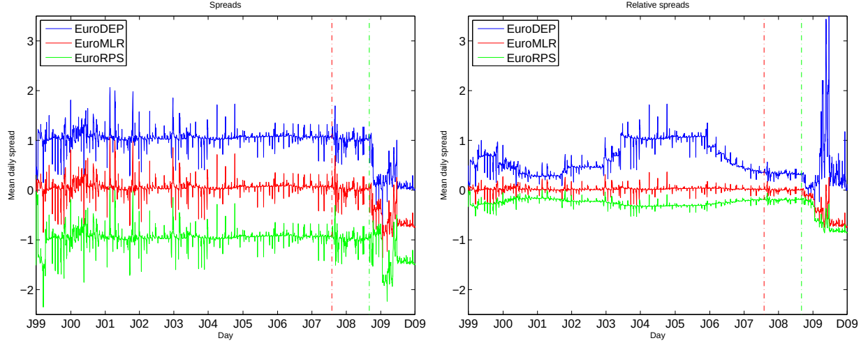
FIG. 3. 1). Left: raw spreads. Right: relative spread (Eq. 2). It is clearly possible to isolate two different behavior; one for the long period before the Lehman collapse, and one for the subsequent period.
