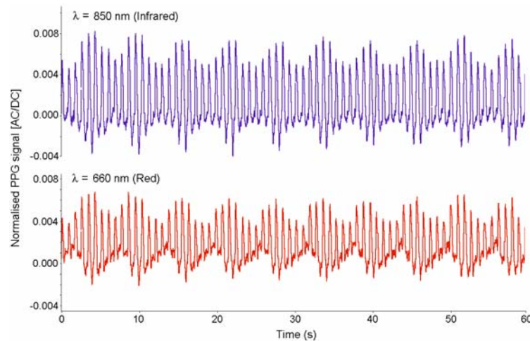
Figure 3. 60-second sample of the normalized infrared and red PPG waveforms obtained at a measurement depth of 20 cm.
