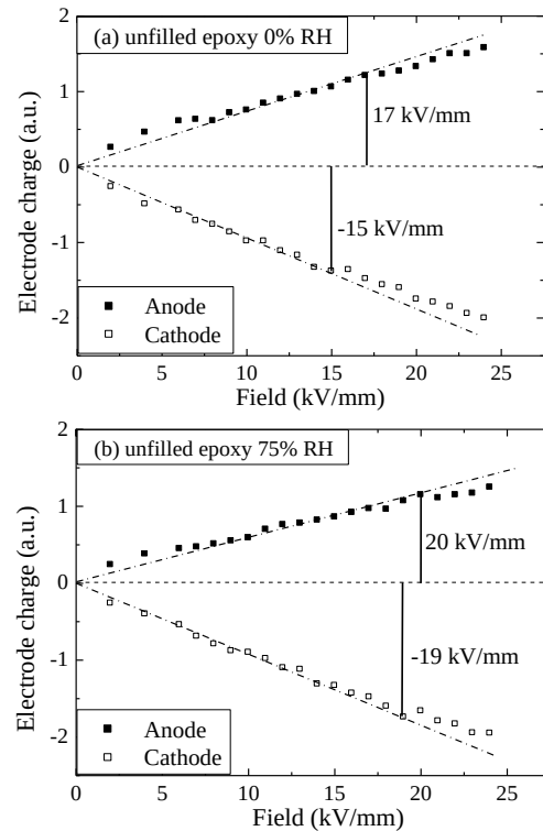
Figure 3: Space charge threshold characteristic of unfilled epoxy at electrodes under various humidities, (a) 0% RH, (b) 75% RH
