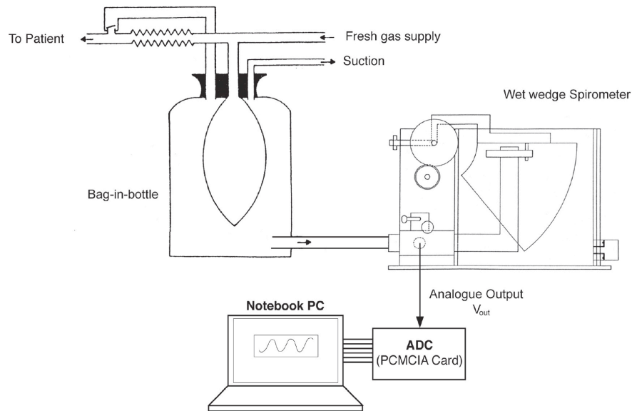
Figure 2. Block diagram of the breathing system.
