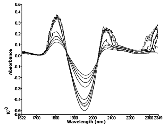
Fig 4. Second derivative spectra of porcine skin undergoing desorption after 30 minutes of hydration time.
