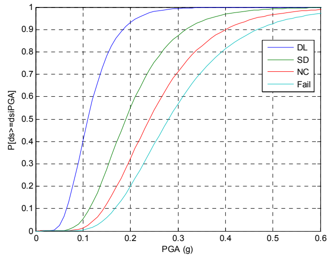
Figure 7. PGA fragility curves for the pristine R/C school building
