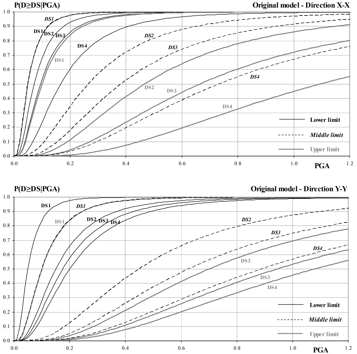
Fig. 15 Fragility curves for the pristine building model
