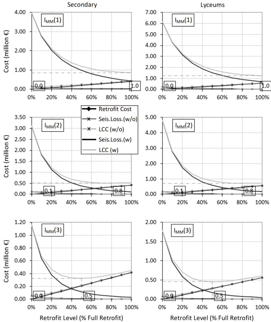
Fig. 21 Life-cycle cost analysis for R/C buildings (secondary, lyceums) for the three seismic hazard relationships
