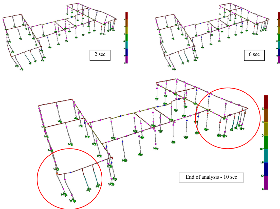
Fig. 14 Damage sequence and localisation at corners
