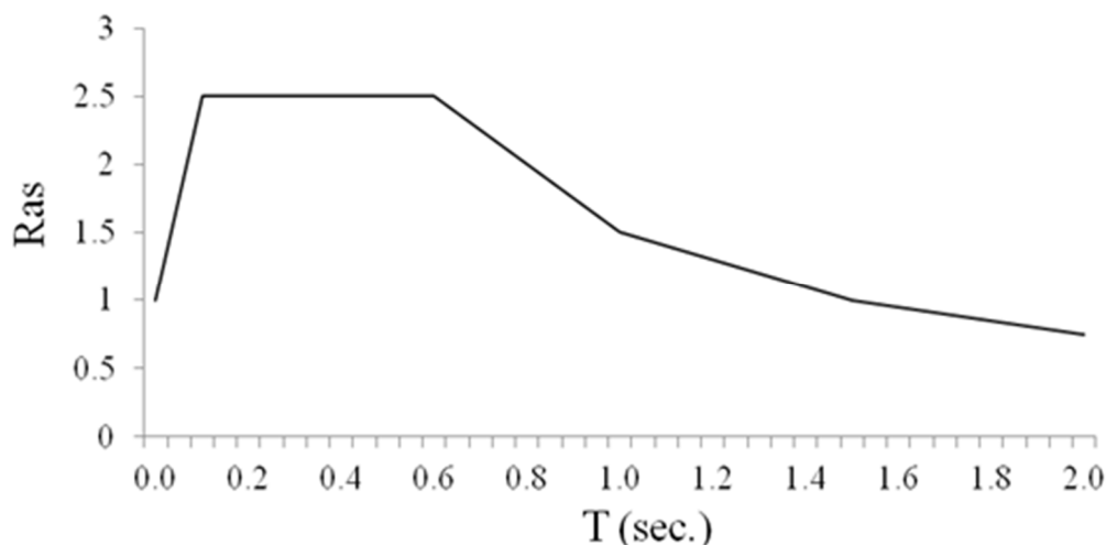
Figure 6. Normalised response spectrum based on the local microzonation study
