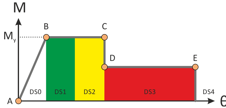
Fig. 12 Definition of damage states
