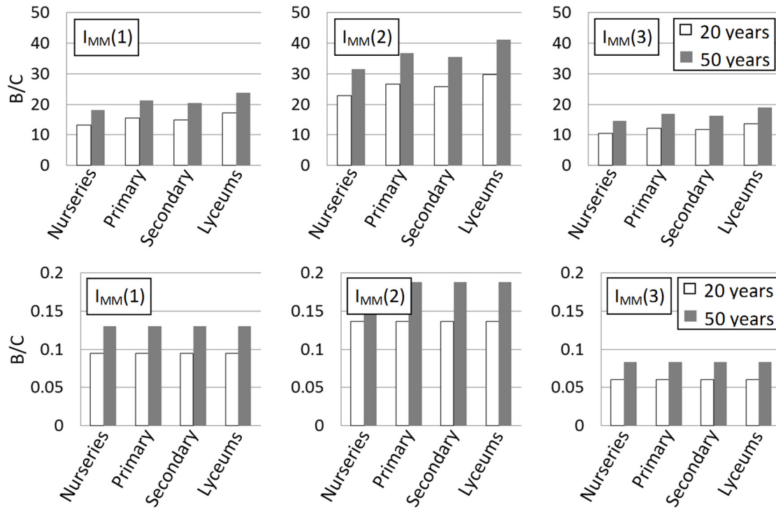
Fig. 22 Benefit/cost ratios for masonry buildings using the lower bound of fragility curves, assuming full diaphragm action after retrofit, with (top) and without (bottom) taking into account the statistical value of human life, for the three hazard relationships ( I_{MM} )
