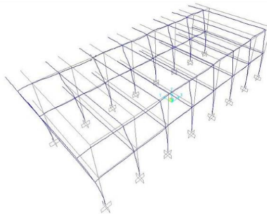
Figure 4. Structural model and fundamental mode shape of R/C building
