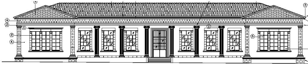
Fig. 9 Masonry school building (elevation)
