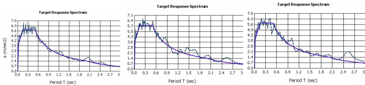
Fig. 11 Elastic response spectra of artificial accelerograms, compliant to EN1998 soil type B.
