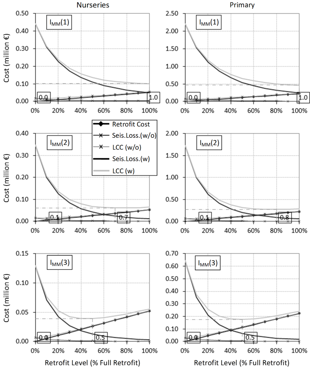
Fig. 20 Life-cycle cost analysis for reinforced concrete buildings (nurseries, primary) for the three seismic hazard relationships
