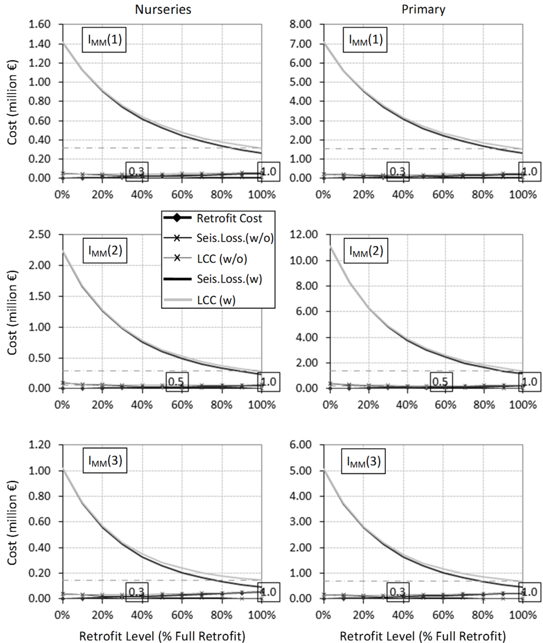
Fig. 23 Life-cycle cost analysis for unreinforced masonry buildings (nurseries, primary) for the three seismic hazard relationships
