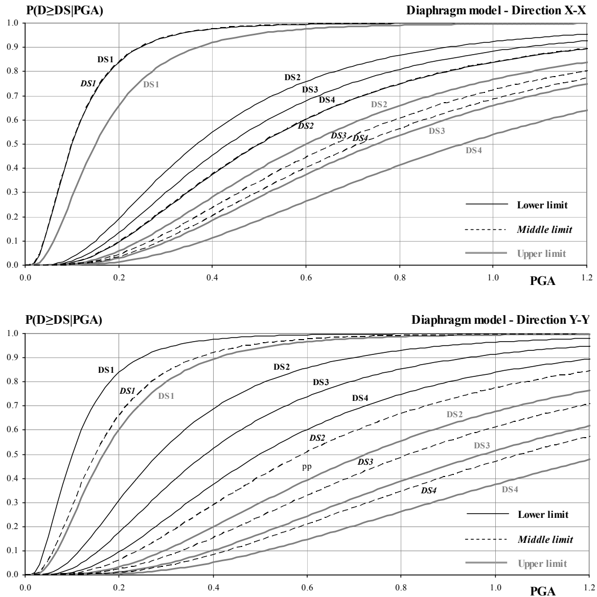
Fig. 16 Fragility curves for the fully strengthened building model (rigid diaphragm)
