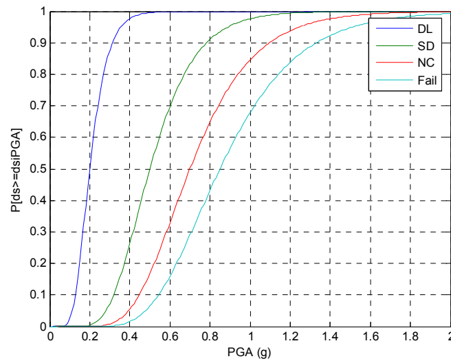
Figure 8. PGA fragility curves for the strengthened R/C school building
