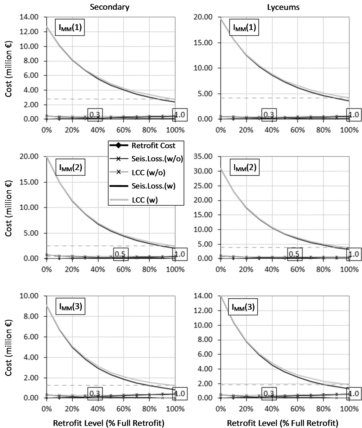
Fig. 24 Life-cycle cost analysis for unreinforced masonry buildings (secondary, lyceums) for the three seismic hazard relationships
