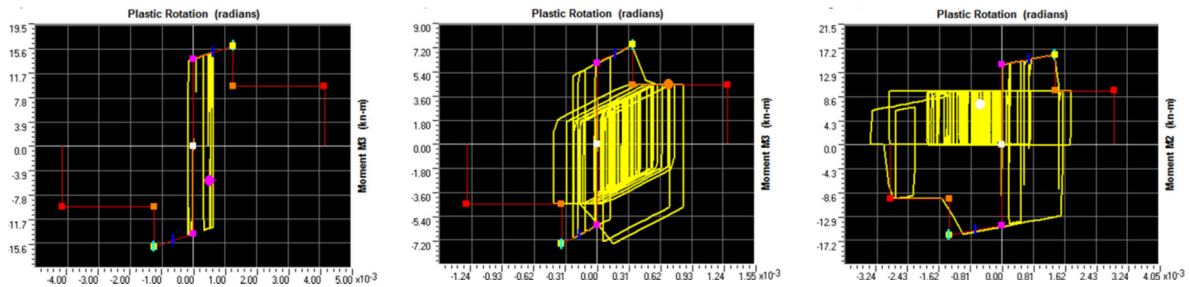
Fig. 13 Cyclic moment vs. plastic rotation response for DS1, DS2 and DS4 damage levels
