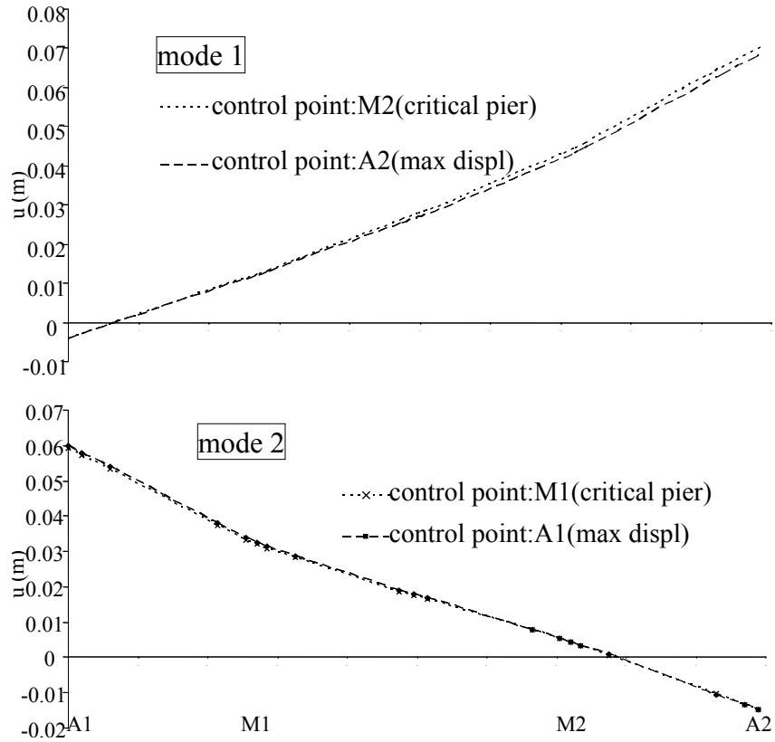
Figure 6: ‘Modal’ deck displacements derived with respect to different control points using u_m' as target displacement according to the improved MPA procedure – overpass bridge ( A_g=0.16g )
