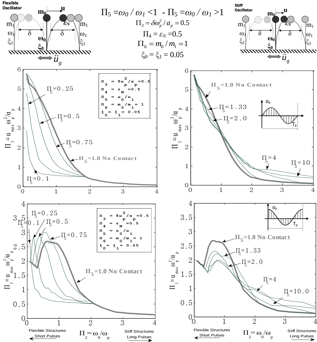
Figure 7 Self-similar response spectra (master curves) for the mechanical system of three SDOF oscillators subjected to, a one sine (top) and one cosine (bottom), acceleration pulse. Left column corresponds to most flexible - right column to most stiff among the two oscillators, and results are showed for several stiffness ratios.
