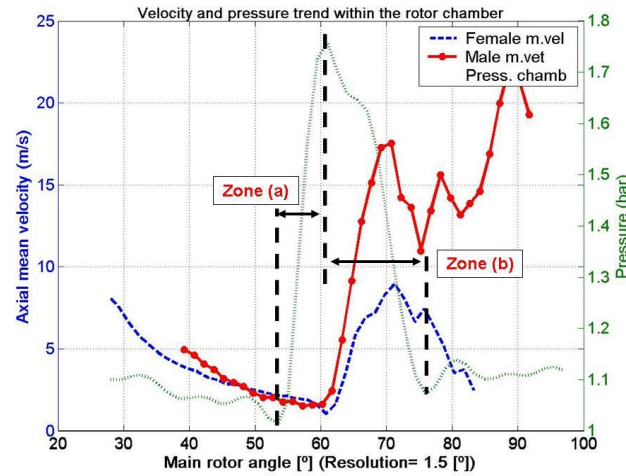
Figure 5 Pressure and velocity distribution within the rotor chamber.
