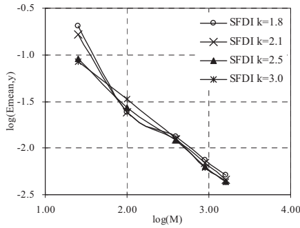
Fig. 13 Convergent rate of the SFDI for estimating the gradient of cosine function (Eq. (15))
