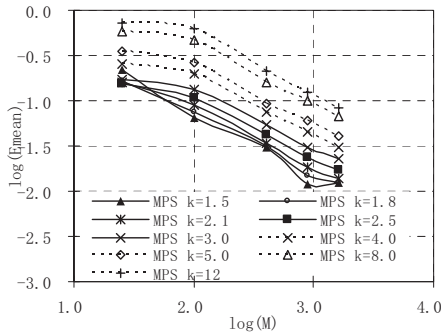
Fig. 8 Convergent rate of the MPS for interpolating the polynomial function (Eq.(5a))
