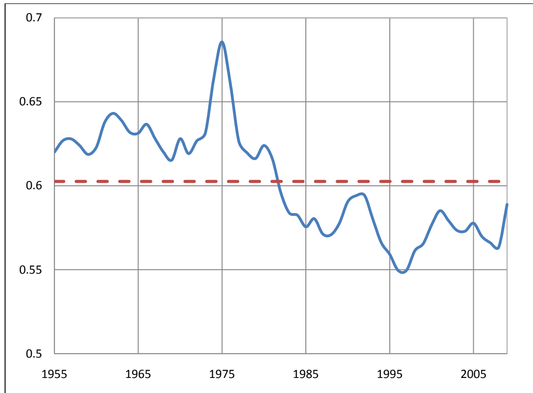
Figure 12 Historical data showing the variation in the wage share of the GDP, \theta , for the UK from 1955. Note the large peak at 1975, during a period of considerable industrial unrest. During this period the mean wage share was 0.603, or about 60%, and the standard deviation was 0.032, so that the coefficient of variation is about 5%.
