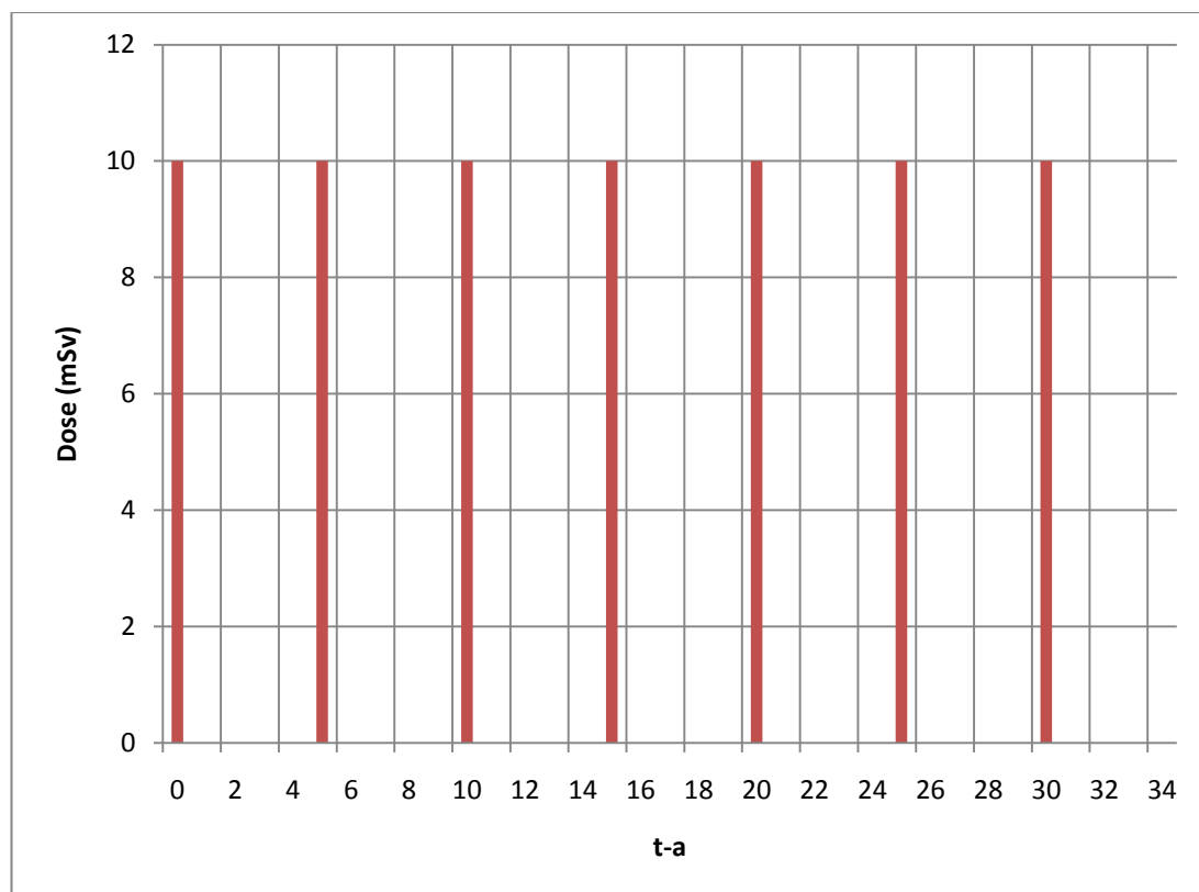
Figure 26 Dose received by individual of age a who is undergoing scans at future age t .
