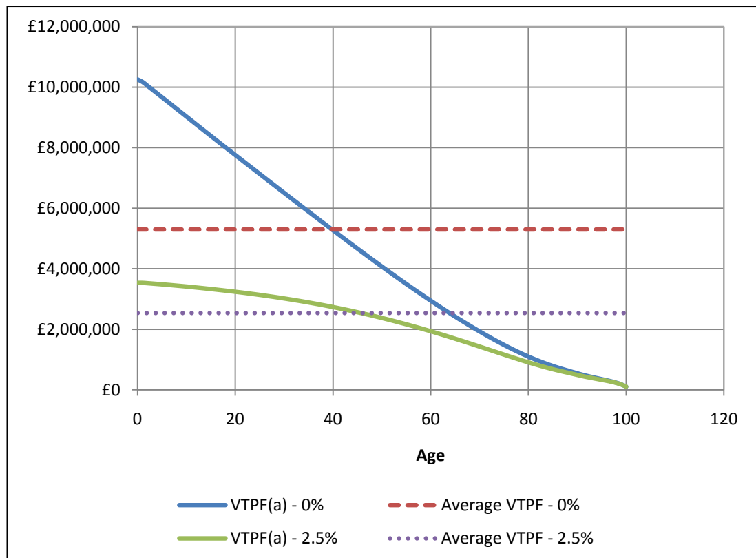
Figure 15 Values of the age dependent VTPF, and the age-averaged VTPF, for discount rates 0% and 2.5%. The average values of the VTPF are £5.3 million and £2.5 million, respectively. These are evaluated at J = 1 .
