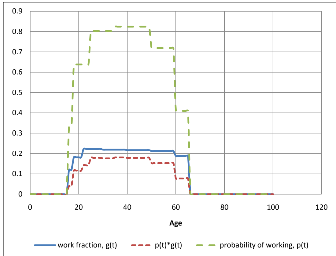
Figure 20 Actual distributions calculated from UK data for 2009 for g_w(t) , p_w(t) and p_w(t)g_w(t)
