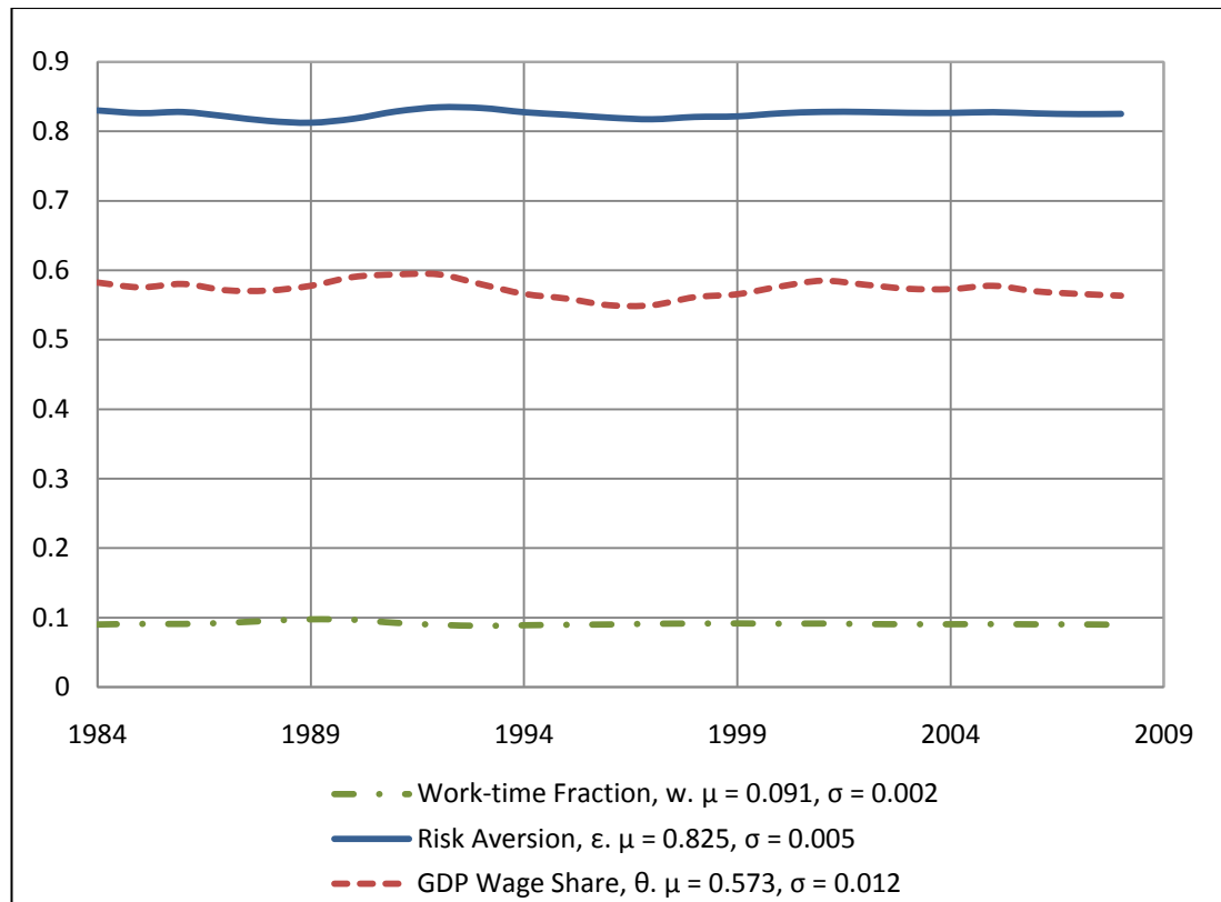
Figure 13 Time series data from the work time fraction, w_0 , the wage share of the GDP, \theta , and the risk aversion, \epsilon , for available data from 1984 to 2008.
