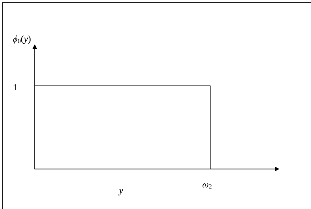
Figure 8 The excess mortality distribution for pollution-induced mortality.
