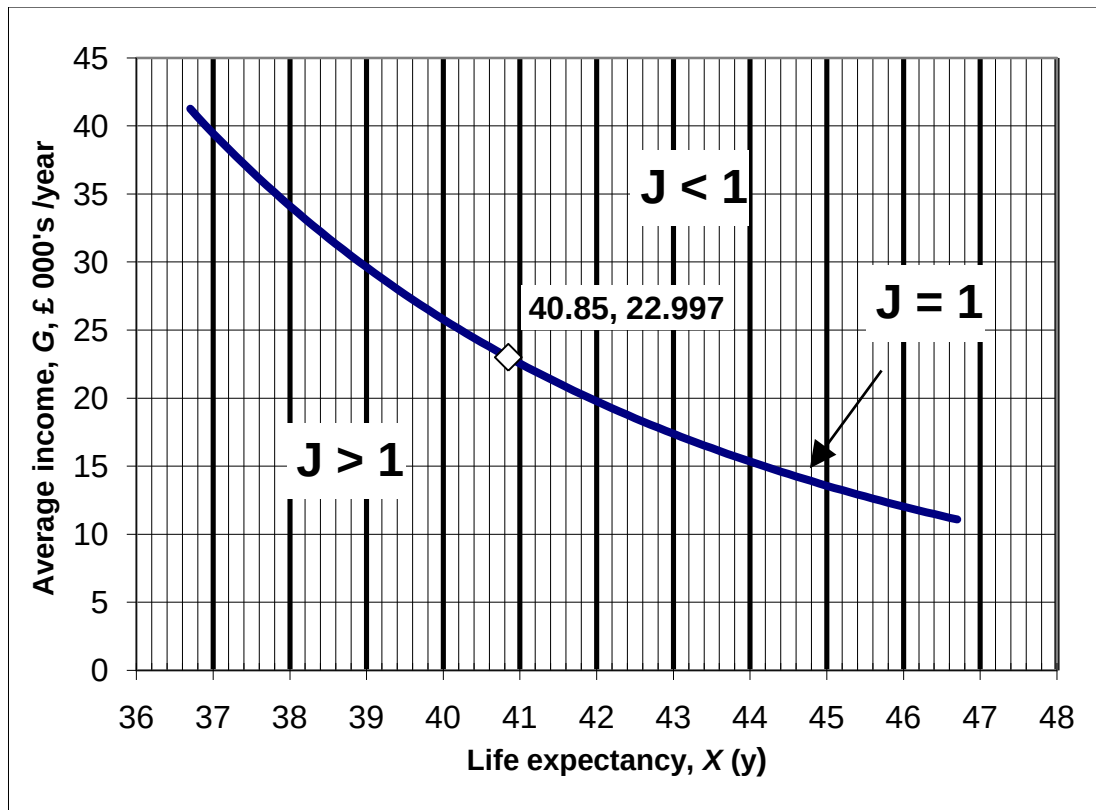
Figure 3 J = 1 indifference curve for income against (undiscounted) life expectancy.
