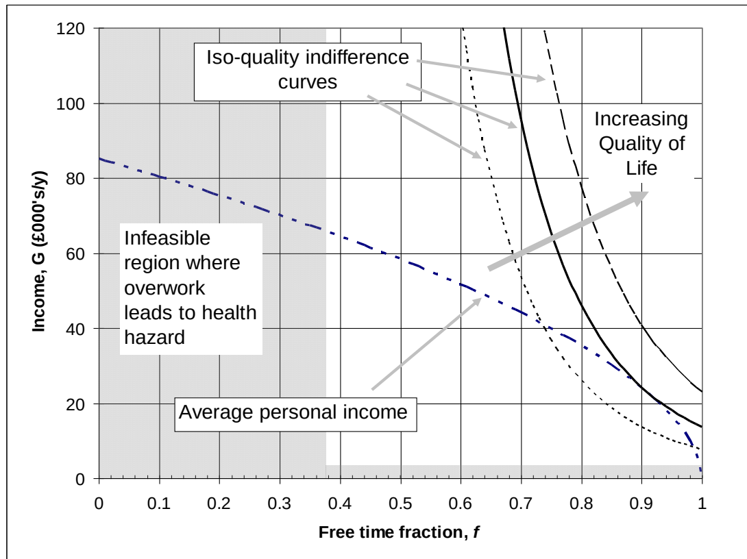
Figure 1 Indifference curves of quality of life against the income constraint.
