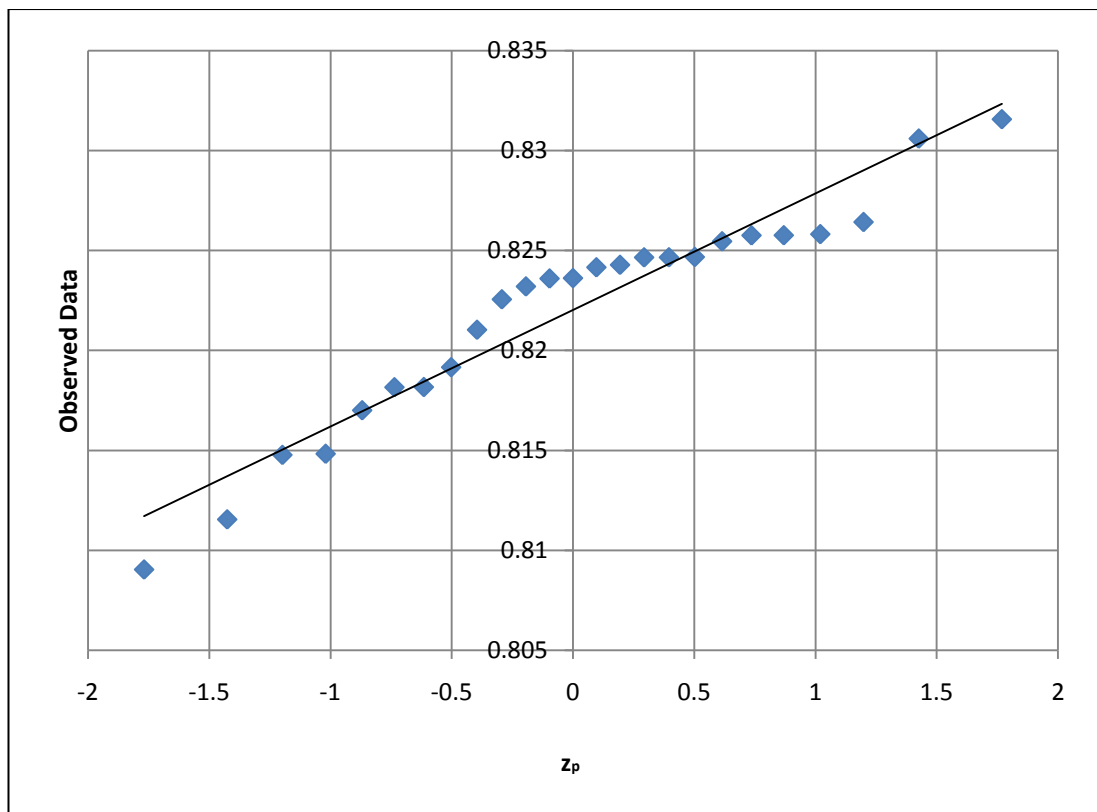
Figure 14 Normal-quantile plot for risk aversion normality test.
