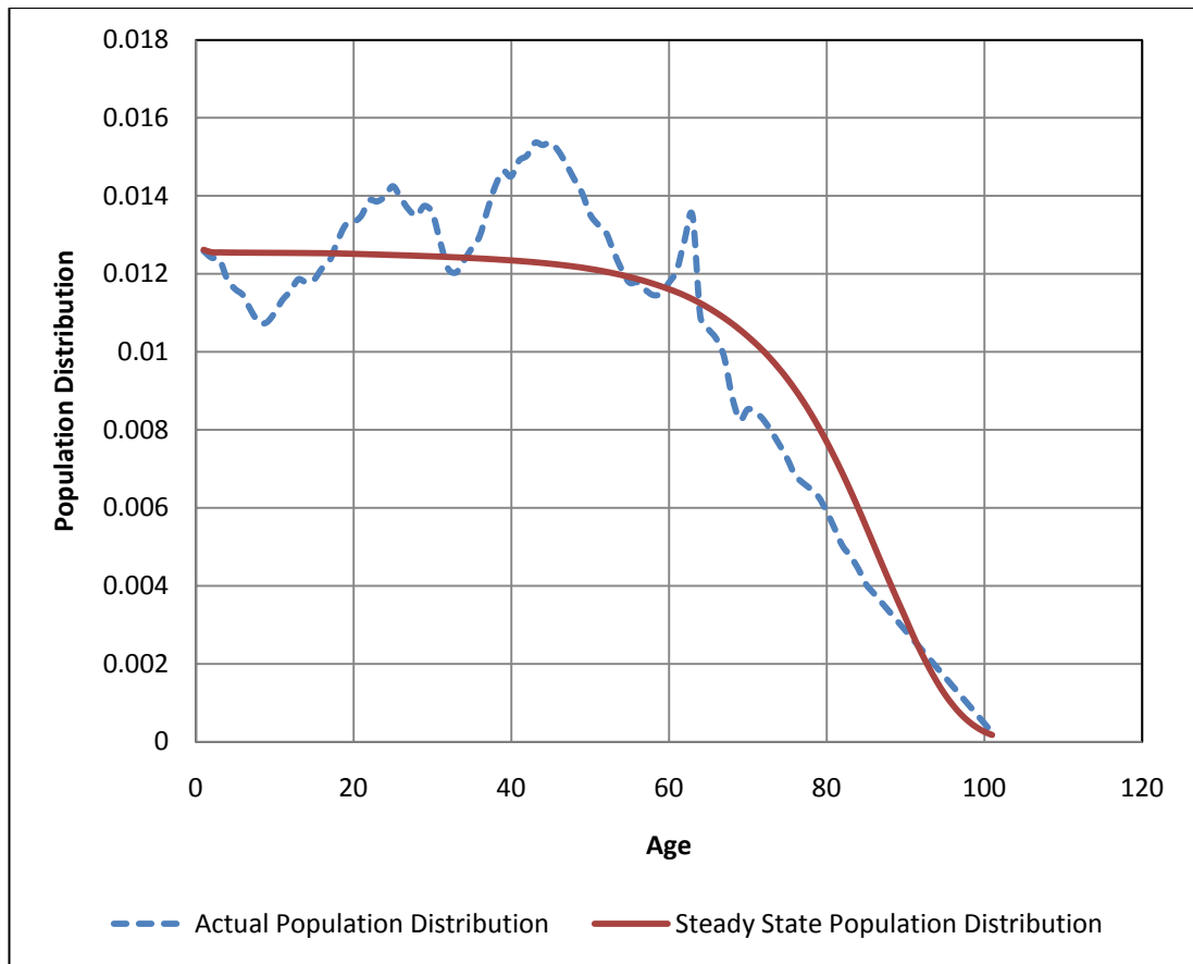
Figure 4 Population distributions calculated from UK data for 2007-2009.
