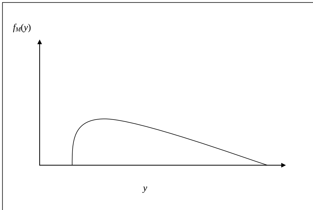
Figure 6 Probability density for the mortality period, y .
