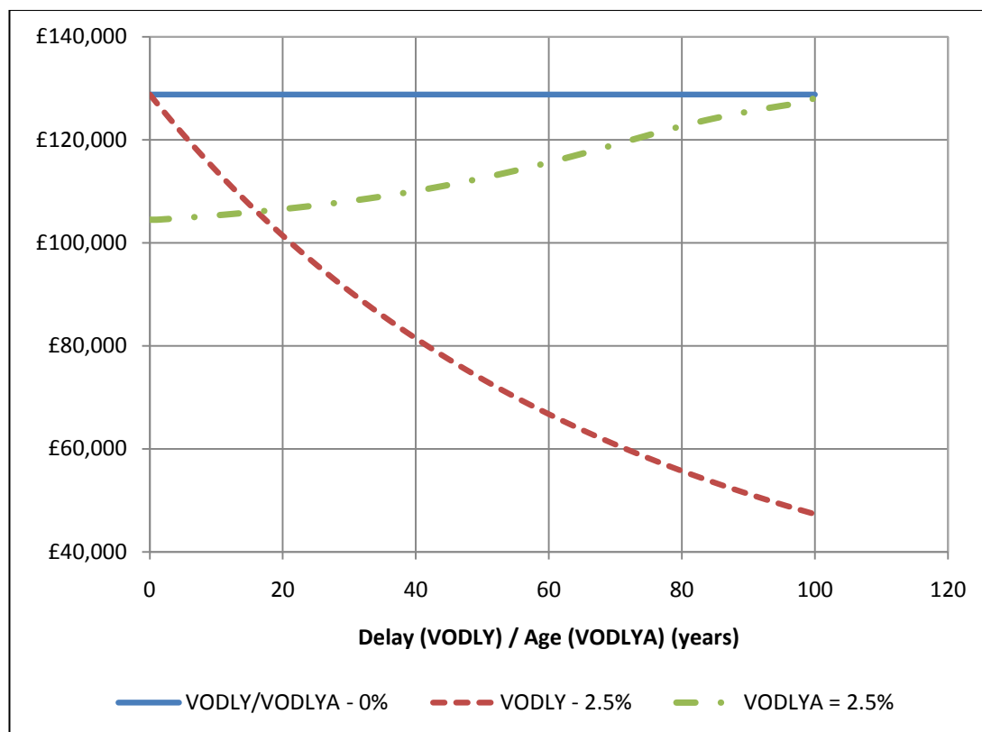
Figure 16 Values of the VODLY and VODLYA, for discount rates of 0% and 2.5%. At 0% discount rate, the VODLY and VODLYA are equal and constant, at about £129,000. The abscissa is for the VODLY is the delay before the life-year is saved, whilst for the VODLYA, the abscissa is the age of the individual.
