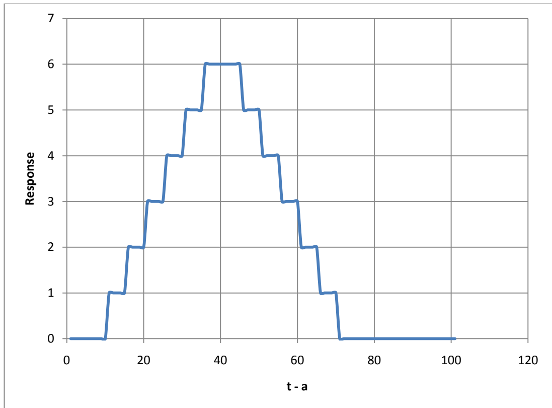
Figure 27 The response of the additional risk faced by an individual of current age a at future age t , following an exposure type given in Figure 26.
