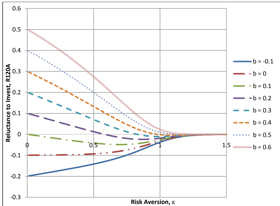
Figure 21 Response of the reluctance to invest ( R_{120A} ) with increasing risk aversion ( \varepsilon ), for different normalised costs of the safety system ( -0.1 < b < 0.6 ). Assets ( A ) are £180,000, normalised accident cost ( c ) is 0.995, and the probabilities of no accident with and without the safety system are p_2 = 1 and p_1 = 0.9 respectively.
