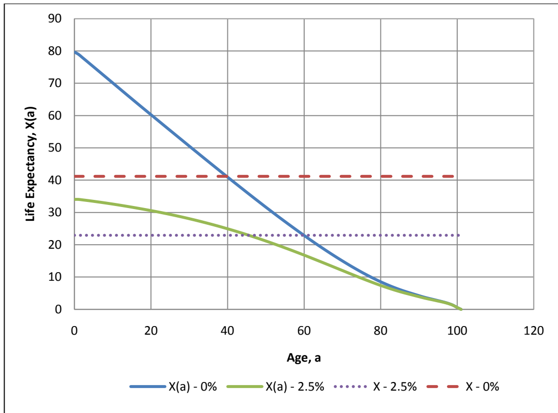
Figure 11 Life expectancy, X_d(a) , and average life expectancy, X_d , for discount rates of 0% and 2.5%. Assumed 50% male female split at all ages. Average life expectancies are 41.2 and 22.9 years at 0% and 2.5% discount rate respectively.
