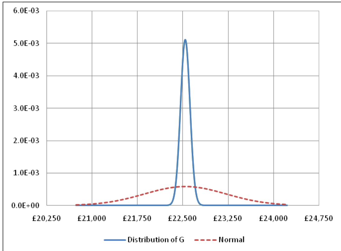
Figure 9 Probability distribution of the GDP per person estimate. Also shown is what the distribution would look like if it were normal.
