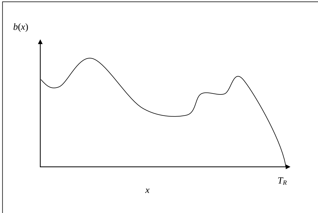
Figure 5 Exposure rate, b(x) , over time, x .
