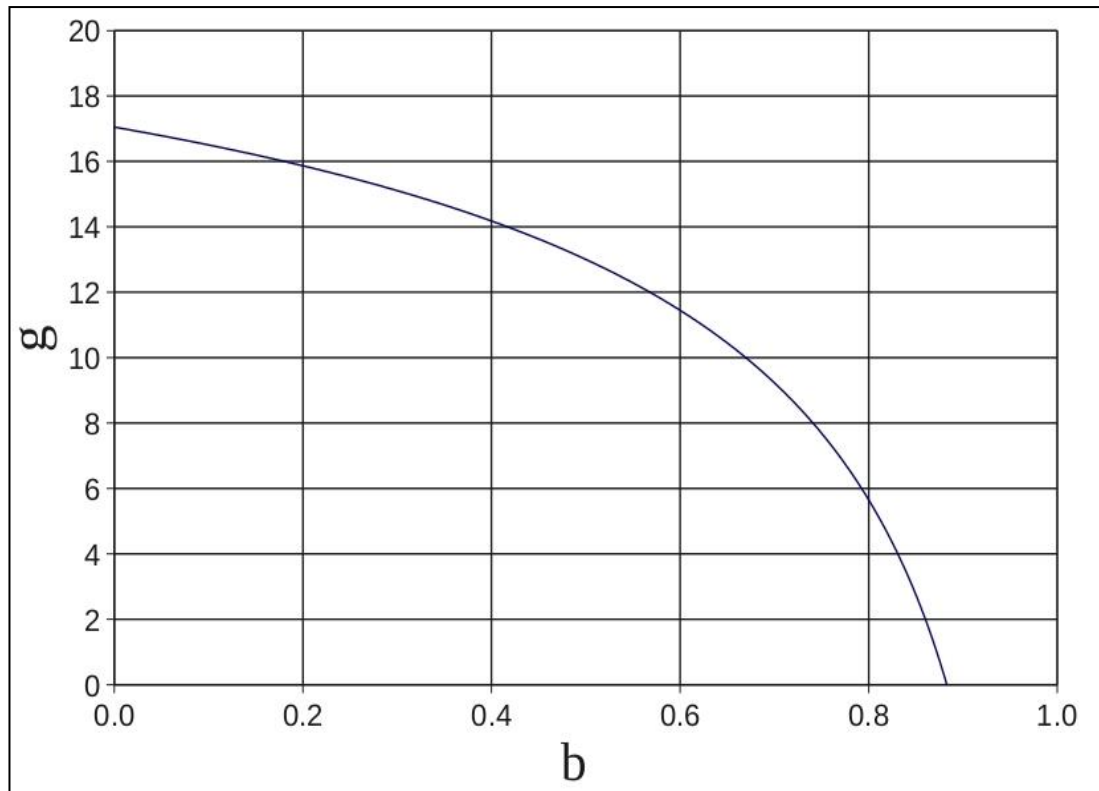
Figure 24 The derivative of the reluctance to invest when \varepsilon = 1.5 and c = 0.9 , illustrating the single root of the objective function g(\varepsilon, b) = 0 . Other parameters are the same as Figure 22
