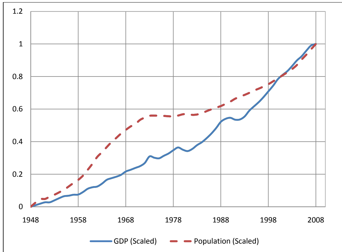
Figure 10 Historical data showing how the UK GDP and population size are correlated. Both are scaled to lie between 0 and 1. At zero, the GDP is about £0.3 billion and the population is about 50 million. At unity, the GDP is about 1.3 billion, and the population is about 62 million.
