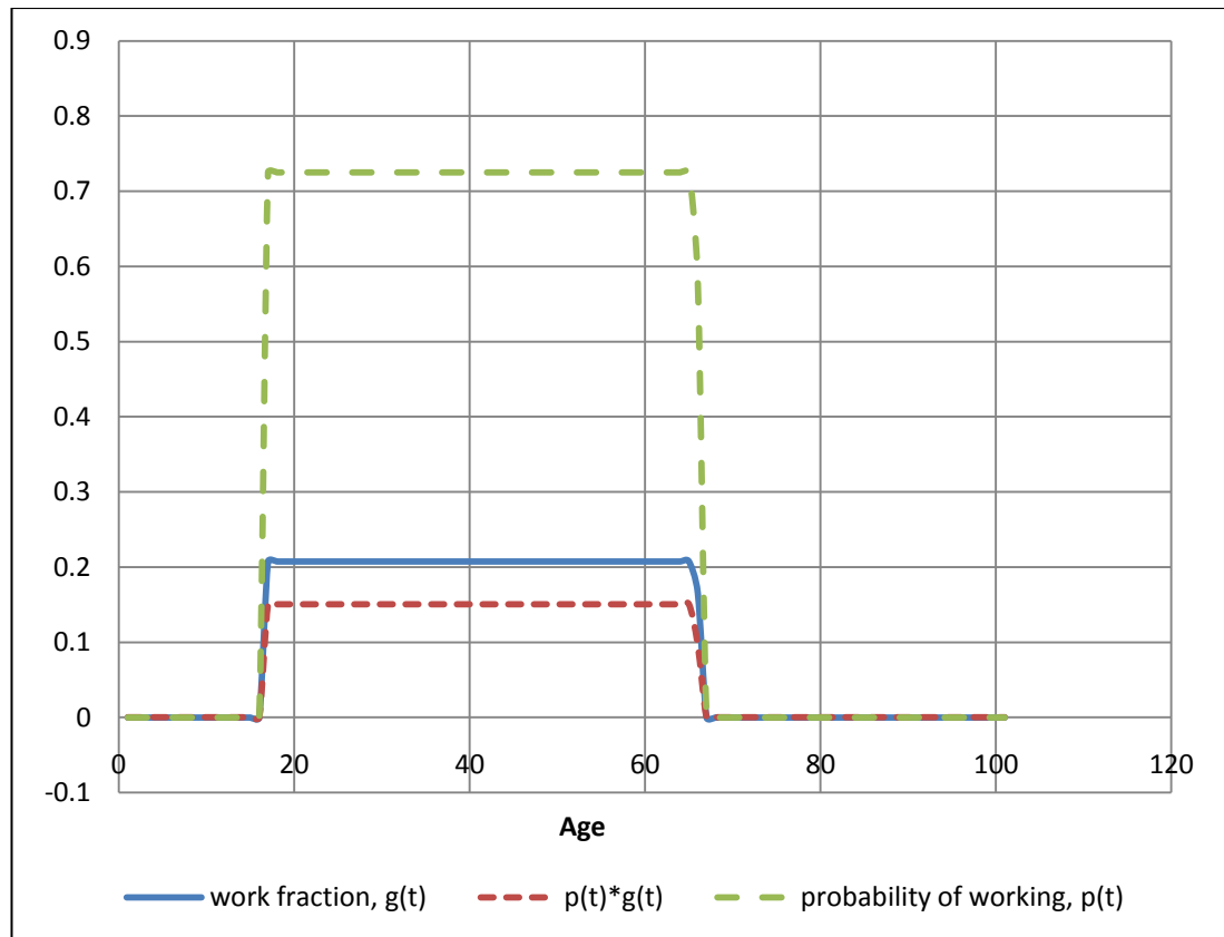
Figure 19 Rectangular distributions for g_w(t) , p_w(t) and p_w(t)g_w(t)
