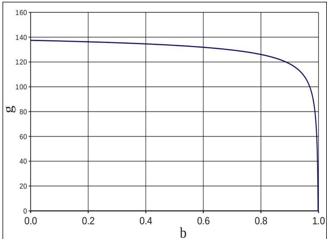
Figure 25 The derivative of the reluctance to invest when \varepsilon = 1.5 and c = 0.999 , illustrating the single root of the objective function g(\varepsilon, b) = 0 . Other parameters are the same as Figure 22. Note the steep gradient in the region around the root.
