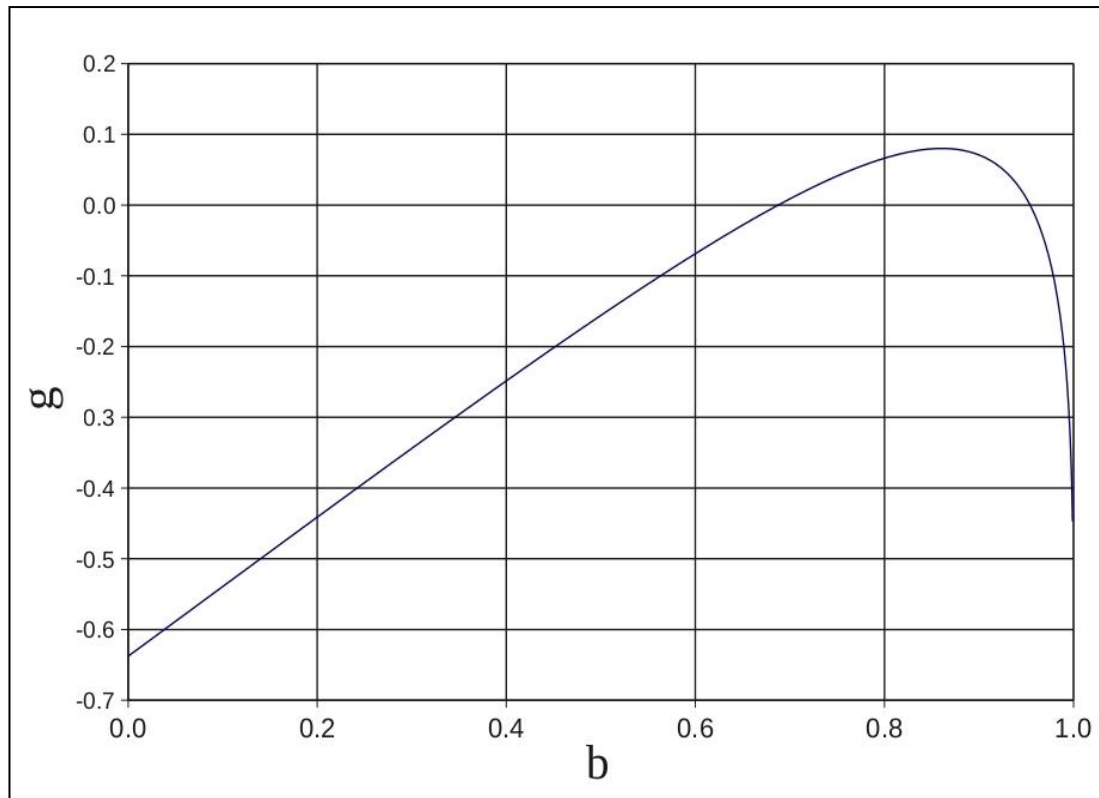
Figure 22 The derivative of the reluctance to invest when \varepsilon = 0.5 and c = 0.9 , illustrating the two roots of the objective function g(\varepsilon, b) = 0 . The assets are A = \text{£}180,000 and all accident probabilities are considered.
