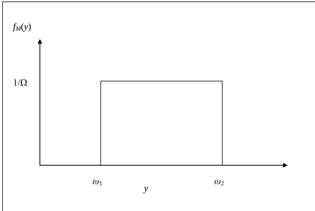
Figure 7 The excess mortality probability distribution for radiation-induced cancer.
