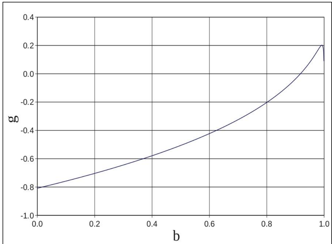
Figure 23 The derivative of the reluctance to invest when \varepsilon = 0.9 and c = 0.999 , illustrating the two roots of the objective function g(\varepsilon, b) = 0 . Other parameters are the same as Figure 22. Note the steep gradient in the region around the second root.
