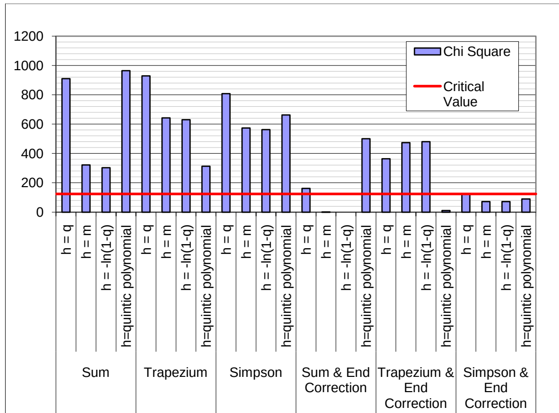
Figure 17 Result of Pearson's chi-square test for 24 tests of: 1. three methods of integrating the cumulative hazard rate (sum, trapezium and Simpson). 2. four different approximations to the hazard rate ( q , m , -\ln(1-q) and a quintic polynomial), and 3. the effect of using the end correction for the final age band. The lower the chi-square value, the closer the empirical data is to the model. The tests that are greater than the critical value (red line) can be rejected.
