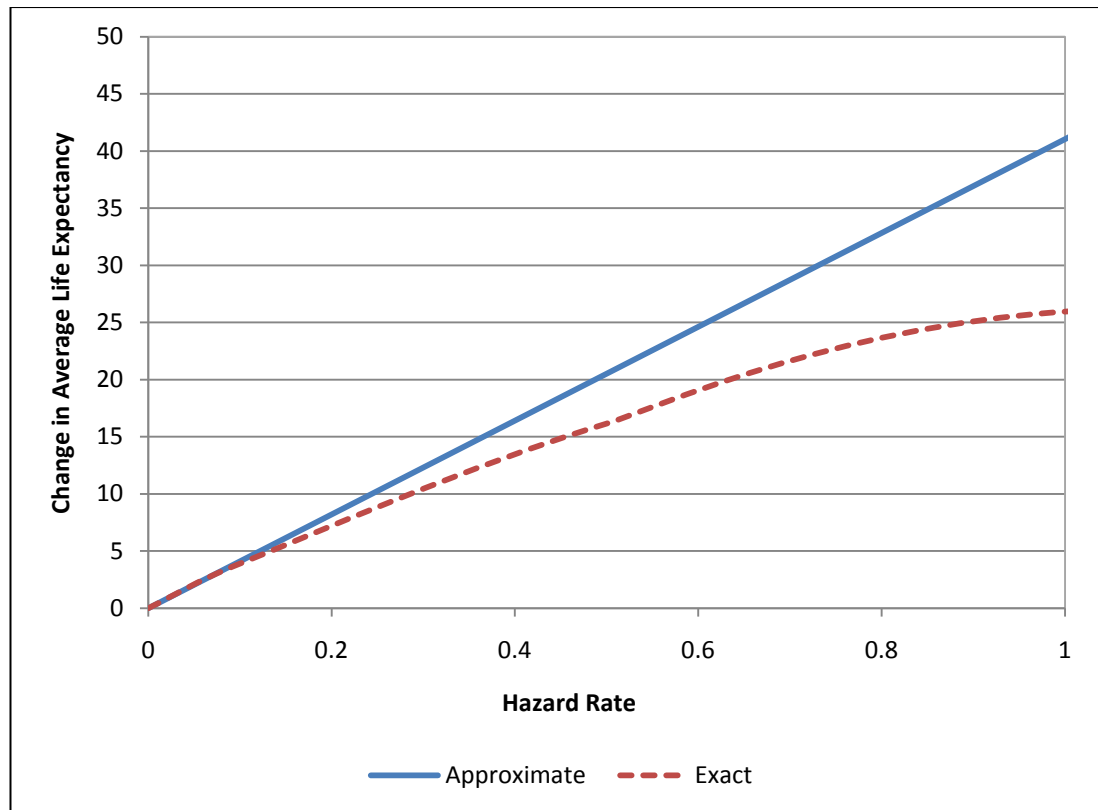
Figure 18 Difference between the linear approximation and the exact calculation of the change in life expectancy, as a function of the hazard rate. The difference between the two is around 5% at a hazard rate of 0.1 \text{ year}^{-1} , and is nearly 30% at a hazard rate of 0.5 \text{ year}^{-1} .
