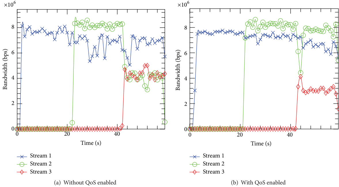
FIGURE 13: Conflict evaluation with and without QoSILAN QoS enabled.
