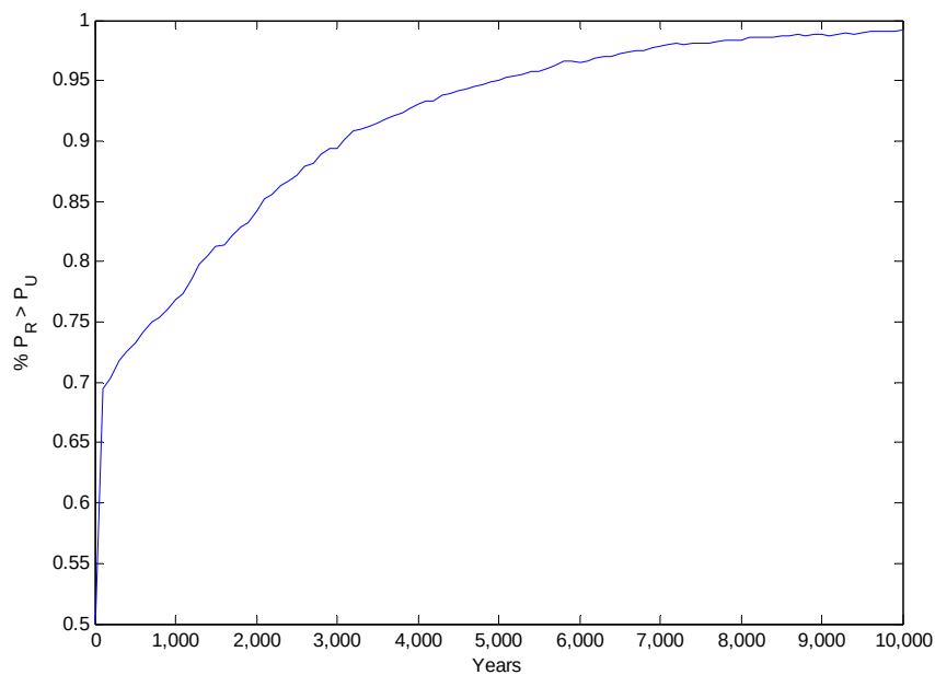
Figure 5.7 Proportion of Outcomes where P_r > P_u This chart shows the proportion of the simulated paths for which the terminal wealth of the rebalanced portfolio P_r is greater than the unrebalanced portfolio P_u . This proportion is shown for simulations with a wide range of different time horizons. The parameters of the simulated values are the same as for Figure 5.6.
