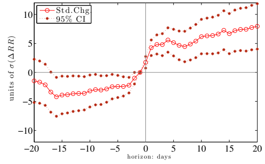
(b) FXRR: 2( moderate ) \rightarrow 1( polarized )
