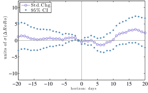
(a) RoRo: 1( polarized ) \rightarrow 2( moderate )
