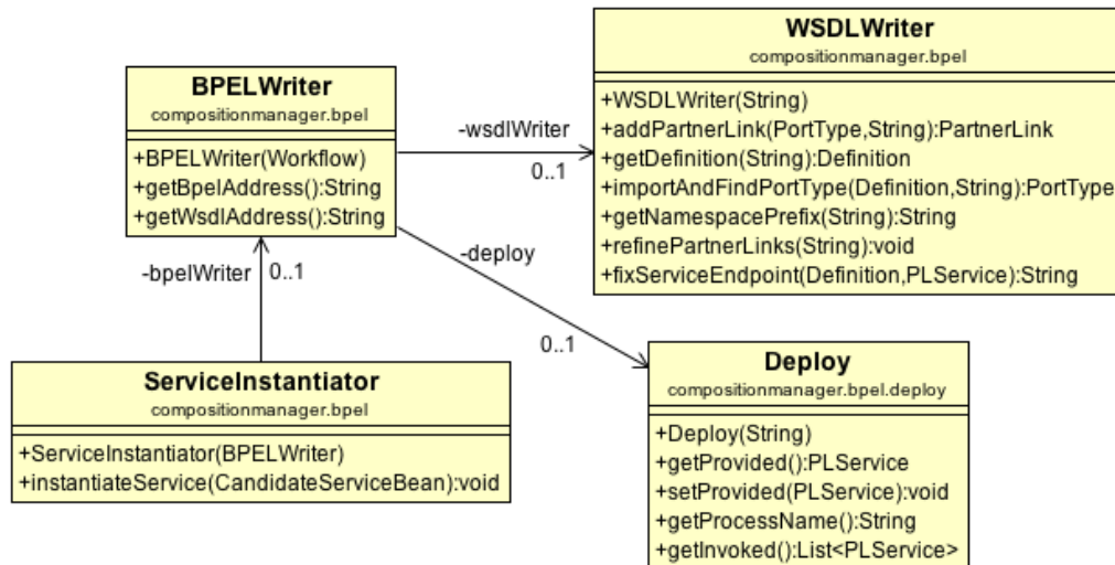
Figure 7.5: Class Diagram of the package compositionmanager.bpel
