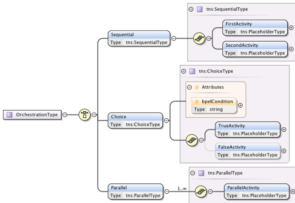
Figure 6.3: The OrchestrationType type of the abstract workflow schema
