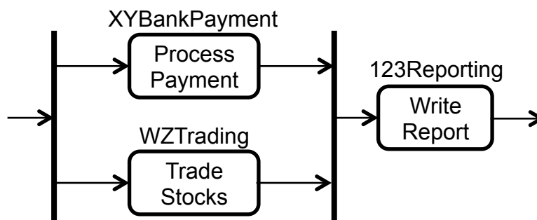
Figure 6.7: Services used by the ProcessOrder SBS
