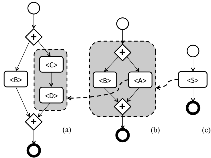
Figure 5.1: Example of workflow pattern recursion
