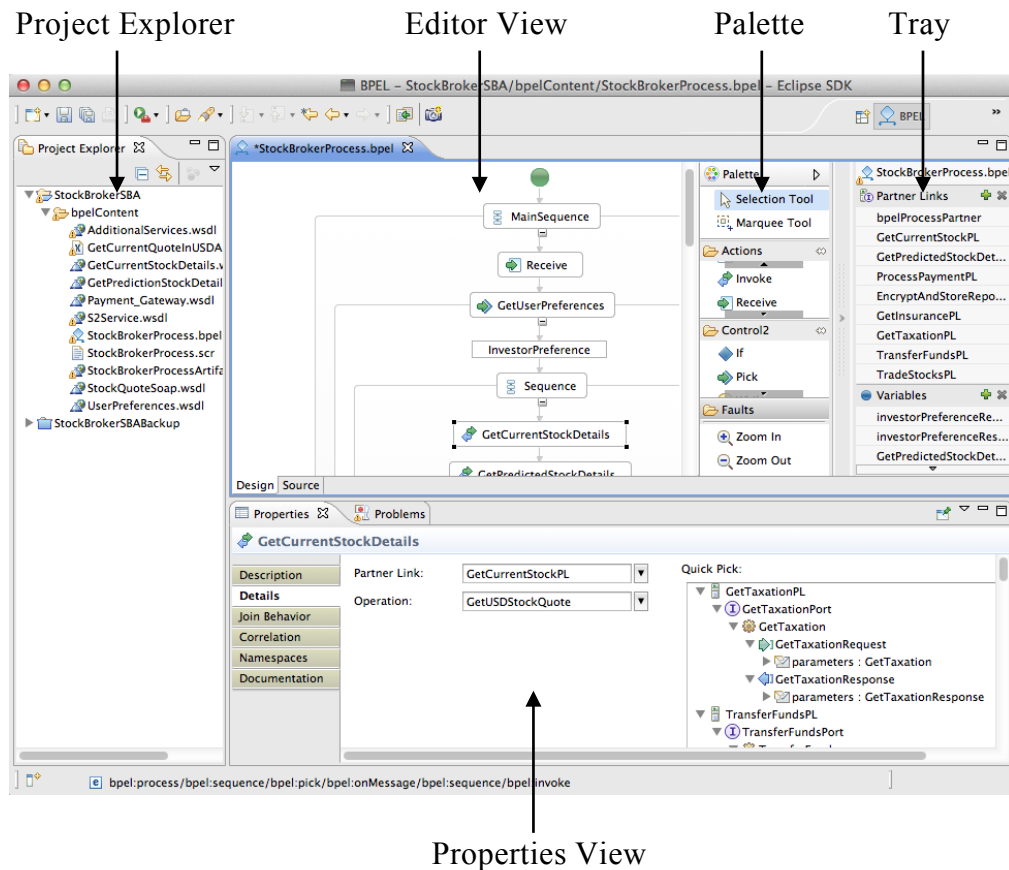
Figure 4.3: Screenshot of the BPEL Designer
