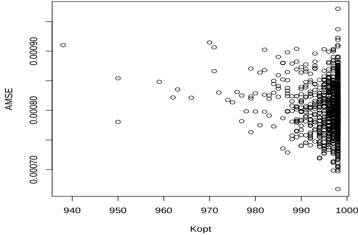
Figure 1: Plots of AMSE(Kopt) against Kopt for Gamma(1.2, 1) .
