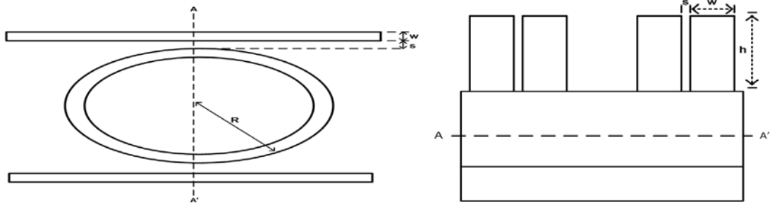
Figure 2.10 (a) Schematic top view of the slot-waveguide based micro ring resonator (b) Cross-sectional view of the slot-waveguide based micro ring resonator
