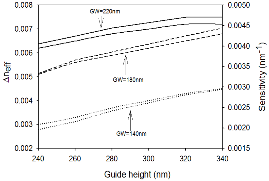
Figure 5.17: Variation of effective index difference, \Delta n_{eff} and waveguide sensitivity with guide height
