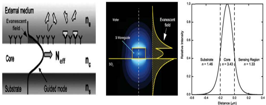
Figure 2.4 (a) Scheme representing evanescent field sensing. (b) A cross section of a silicon photonic waveguide and the optical electric field distribution of the vertically polarized mode are shown. (c) Cross-sectional plot of the evanescent field intensity of optical waveguide [50].
