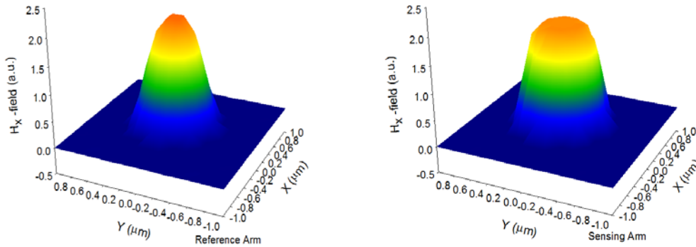
Figure 5.2: (a) 3-D field profile of the H_x mode for the reference and the sensing arm for D = 400 nm
