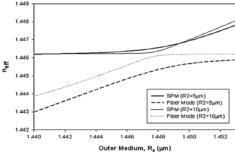
Figure 4.2: Effective index variation with the refractive index of the outer medium, R_4 for the inner and outer SPMs at the gold/cladding and the gold/outer medium interfaces respectively for a cladding thickness of R_2 = 5 and 10\mu\text{m}
