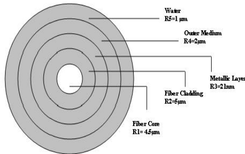
Figure 4.1 Schematic of the SPR structure studied
