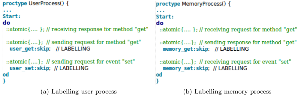
Figure 5.3: Process labels for tracing the executions of shared-data users and memory
