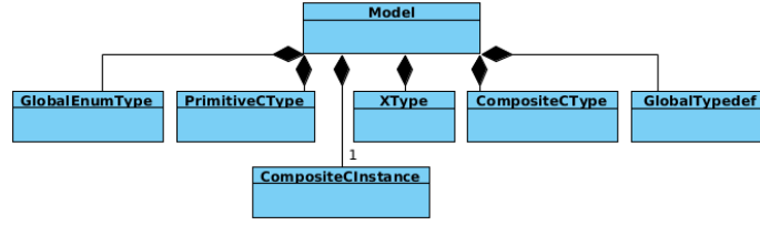
(a) Class diagram of a Model
