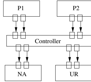
Figure 6.42: Centralised architecture of nuclear power plant
