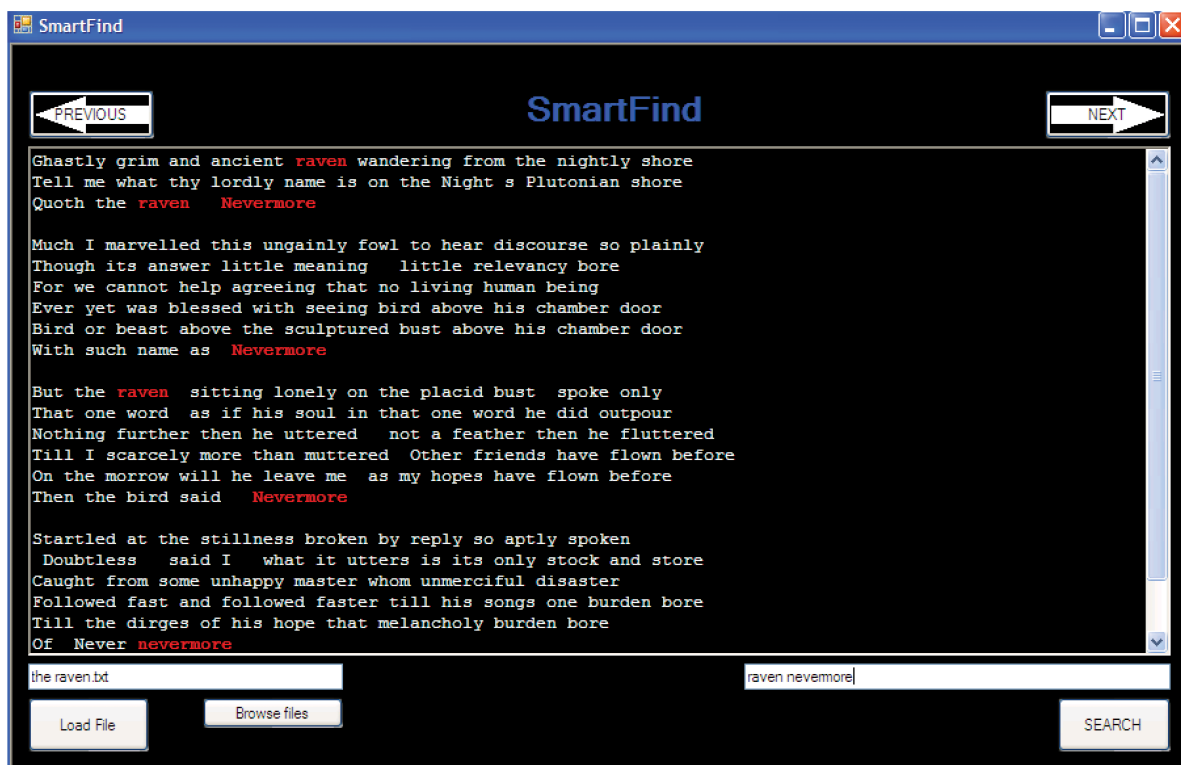
Figure 2.14: SmartFind Tool
