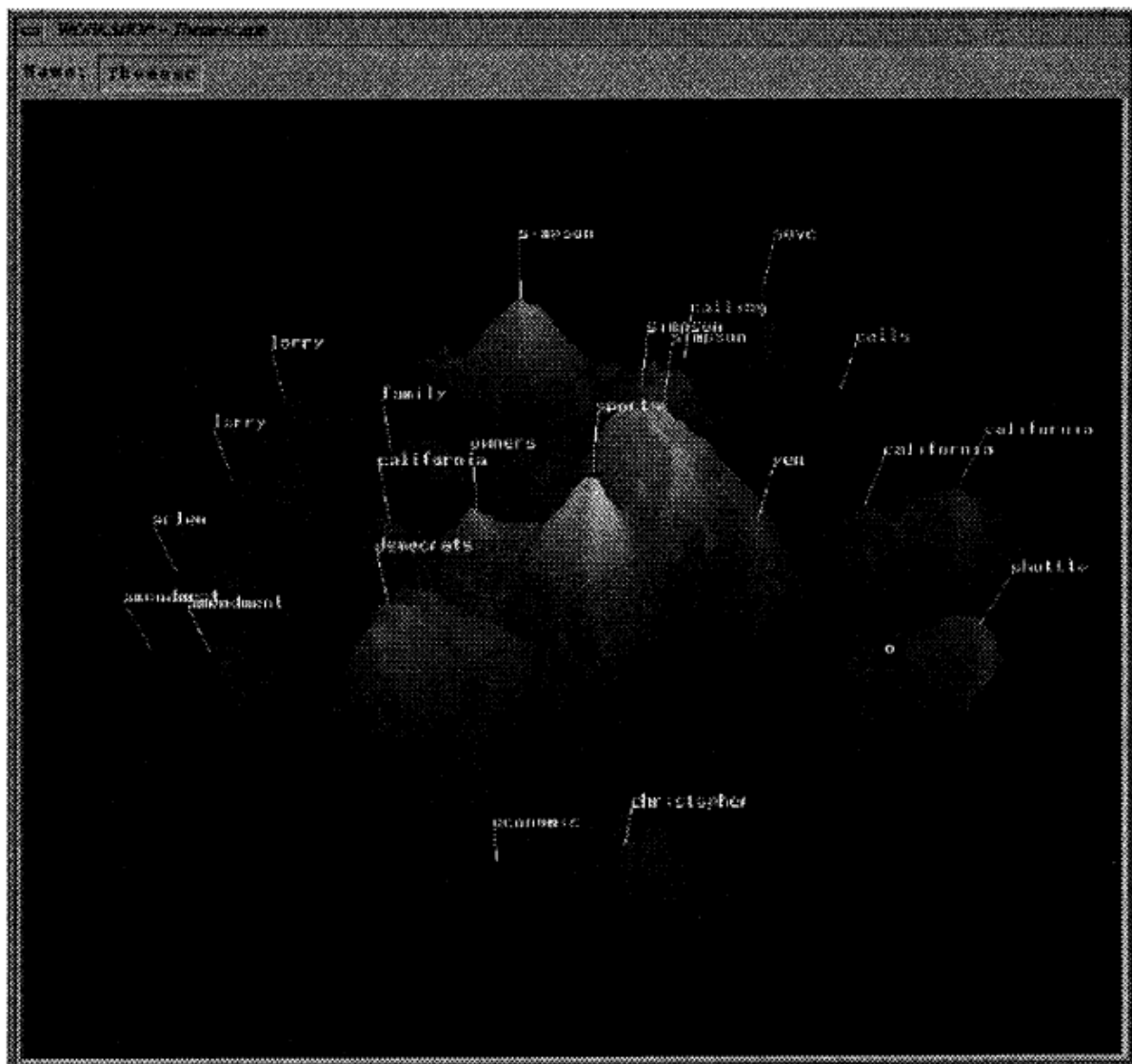
Figure 2.10: Themescape Tool
