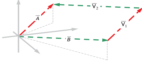
Figure A.1: A vector may be depicted as “an arrow of given length pointing in a given direction”. Given a vector with tail at the “origin” any other arrow that is parallel to this vector, of the same length and pointing in the same direction, is the same vector. This is very useful because any finite dimensional vector space is equivalent to some \mathbb{R}^n and, as such, may be visualised as a collection of arrows.
