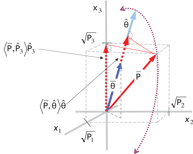
Figure 4.18: The length of the projection of \bar{P} onto a subspace \text{Span}(\theta) , which is the span of an arbitrary difficulty function \theta , is at least as large as the magnitude of \theta , \langle \theta, \hat{\theta} \rangle . This is equivalent to q_{BB} \leq q_B . The case of equality is precisely the case where \theta is a version, such as \bar{P}_3 .
