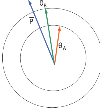
Figure 5.8: We seek a pair of difficulty functions that maximise q_{AB} , with the requirement that one of the vectors touches the sphere of radius \sqrt{q_{BB}} and the other touches the sphere of radius \sqrt{q_{AA}} . From the diagram collinearity of the vectors will give the largest inner-product of the vectors. Since \|\bar{P}\| = 1 it is always possible to define a pair of collinear difficulty functions of the given sizes collinear with the demand profile.
