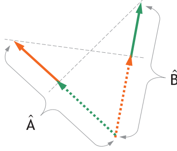
Figure A.5: Unit vectors are projected onto each other
