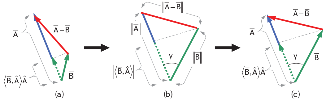
Figure A.7: The inner-product is used to define the angle between two non-zero vectors by creating a 2-dimensional triangle whose sides are the lengths of the relevant vectors. In figure (a) only arrows are used to depict multidimensional vectors in some abstract vector space. In figure (b) a 2-dimensional triangle with sides equal to the lengths of the vectors drawn in figure (a). The angle between the vectors \bar{A} and \bar{B} is the one defined by the angle between the corresponding sides of the triangle in (b); the angle is obtained by employing the cosine rule . Upon having this understanding of the relationship between figures (a) and (b) it is not necessary to depict them as separate; instead, a single picture, such as (c), in which arrows with the corresponding vector lengths separated by the correct angles may be drawn.
