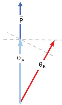
Figure 5.4: Here a pair of difficulty functions, one of them being constant, is assumed to have the same mean (so they have the same projection lengths on the demand profile). The constant difficulty function is parallel to the demand profile, \bar{P} . Consequently, the projection of any other difficulty function in the direction of \bar{P} has a length that is the shared mean and, hence, must be the length of the constant difficulty function.
