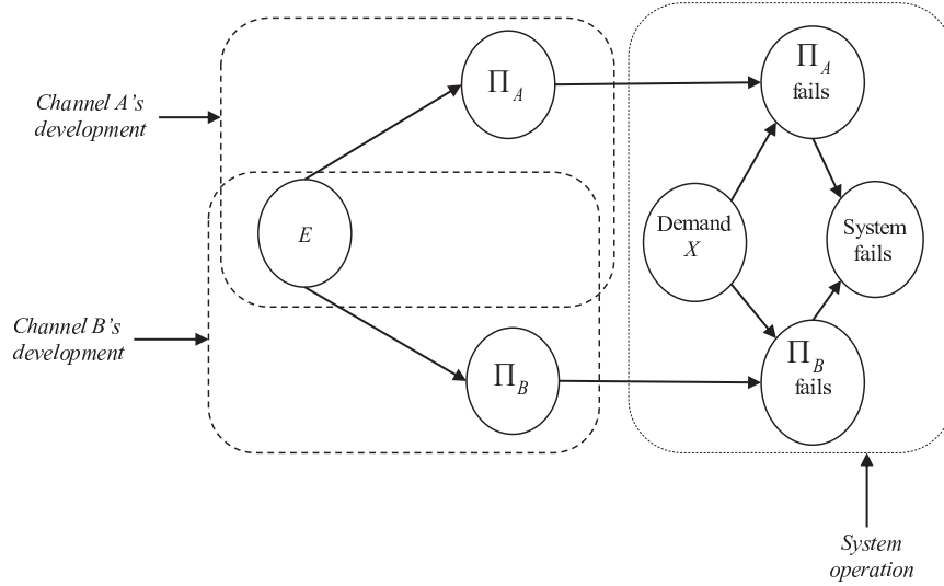
Figure 3.5: Bayesian network for a system with one common influence between the development processes. For example, the same test suite is used to test both versions.
