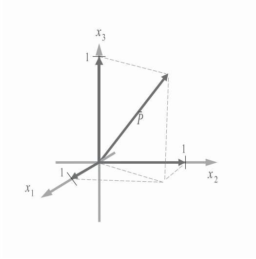
Figure 4.4: “Worst” version, \bar{P} , depicted in terms of the orthogonal basis \mathcal{S} . The vector \bar{P} is a unit vector since its magnitude is 1 (see Eq. (4.9)).
