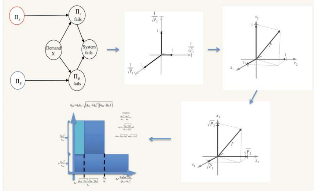
Figure 4.1: A depiction of the 5 steps in extremising expected system pfd : 1) A practical scenario is modeled using the LM model, or any suitable extension thereof (see Chapter 3 for more detail); 2) This, in turn, defines an equivalent vector-space representation; 3) Regions of possible solutions within this vector-space are determined by the constraints of the problem; 4) Computations to derive the bound are simplified by a change in how the vectors are represented (a so-called change of basis vectors ); 5) The bound is obtained and the solution is recast from being in terms of the vector-space, into an equivalent form under the LM model (extension).
