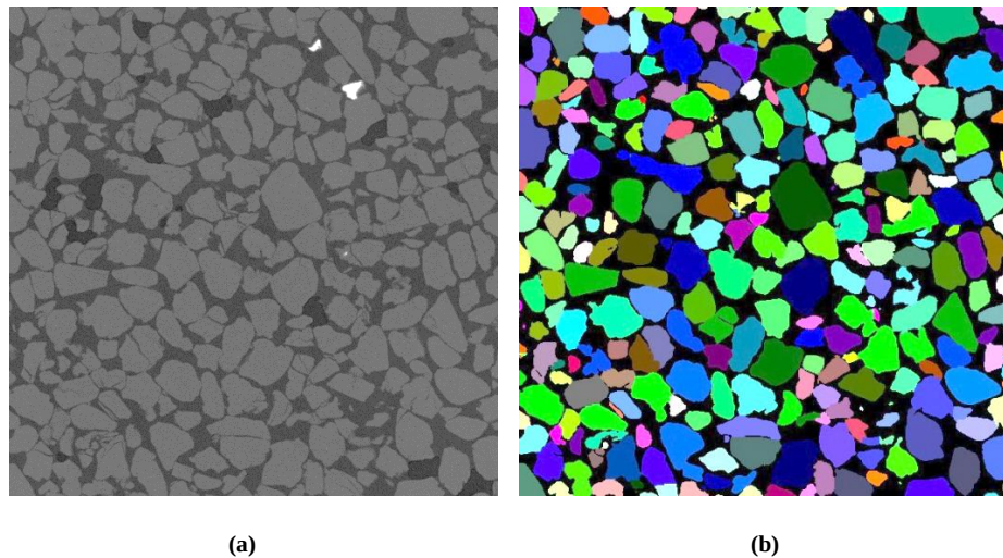
Figure 2. (a) \mu CT raw image and (b) segmented image.
