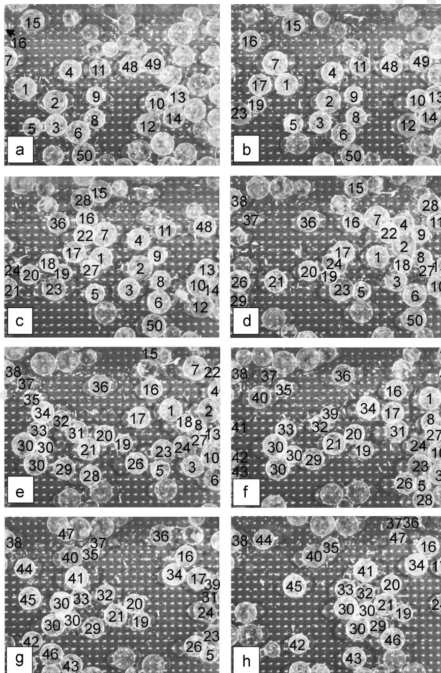
Fig. 3. Image sequence showing the particle motion in the suspension under shear load of the slurry (flow is from left to right). Recorded with 12 fps at 1600 \times 1200 \text{ px}^2 . The figure shows every twelfth picture.
