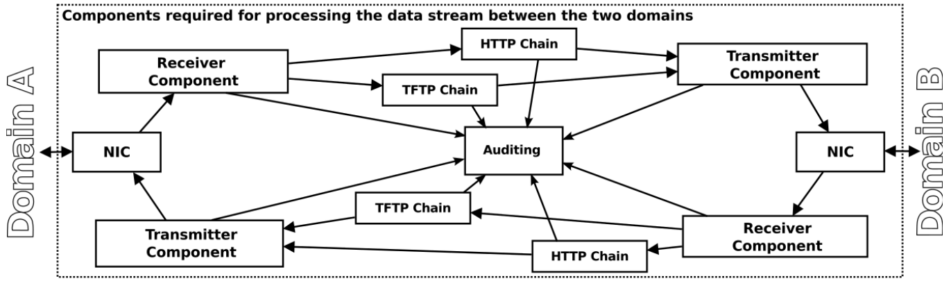
Figure 1: High-level View of Gateway Components
