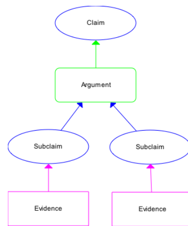
Figure 4: Example of CAE structure in an assurance case
