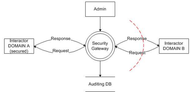
Figure 2: The high-level data flow diagram of the system
