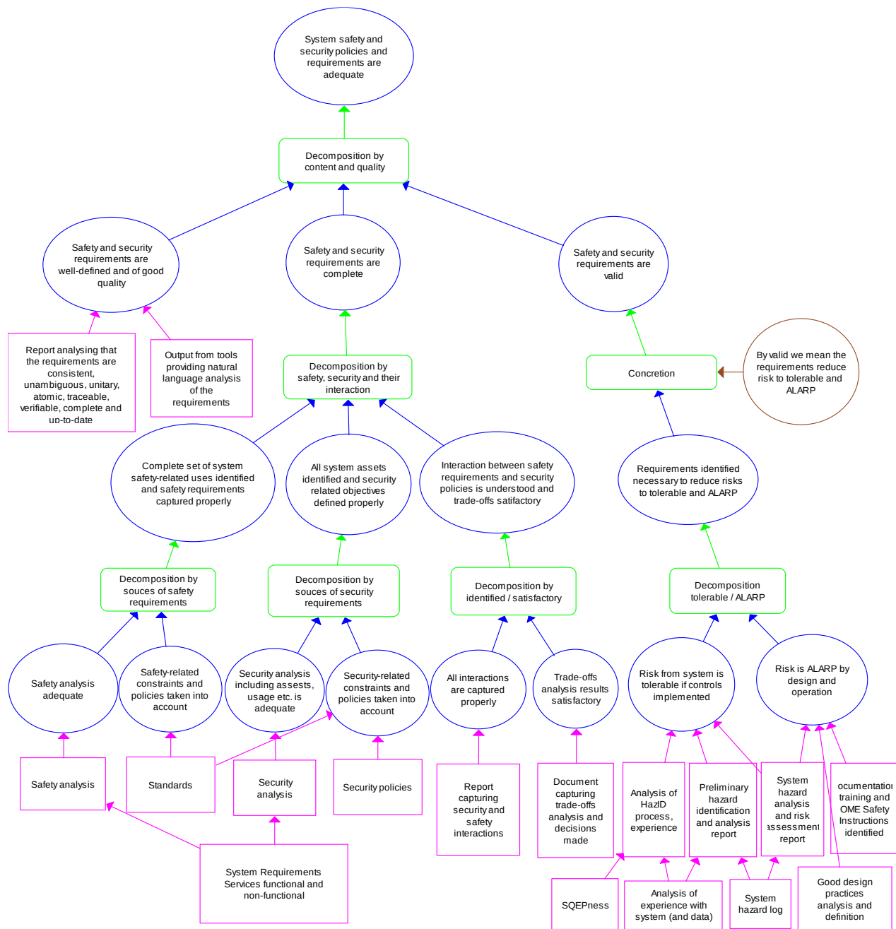
Figure 4. L0-level case fragment for the gateway in CAE notation
