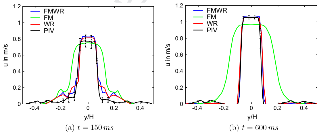
Fig. 18. Development of u(y/H) along baseline P2, comparison of PIV measurement with CFD model results from simulations with CNE and \Delta t_2 .
