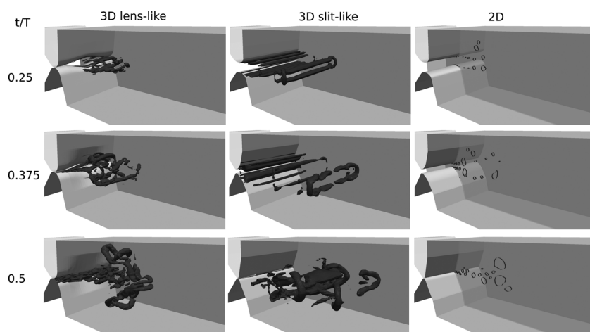
Fig. 4. Vortical structures visualized by iso-value of Q -criterion (iso-value=2000) at certain times t/T during cycle for the simulation runs with 3D lens-like shaped constriction, 3D slit-like constriction and the 2D case, with a constriction that equals the mid-cross section (XY) of the two 3D cases.
